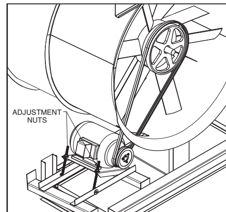
Figure 7 – PM Style Motor Adjustment
