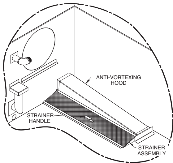
Figure 10 – LSTE/PMTQ Strainer Assembly
