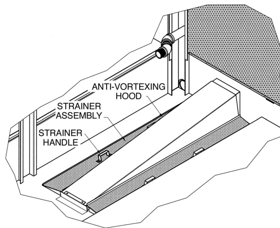
Figure 9 – Dual Strainer Assembly
