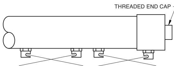
Figure 13 – LSTE/LPT Water Distribution
