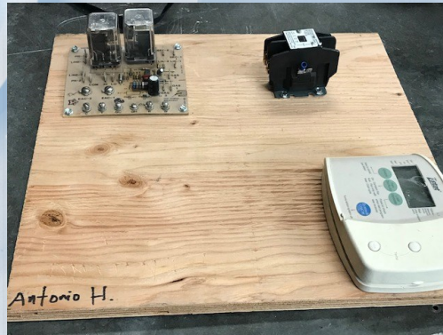
A student's thermostat circuit board
