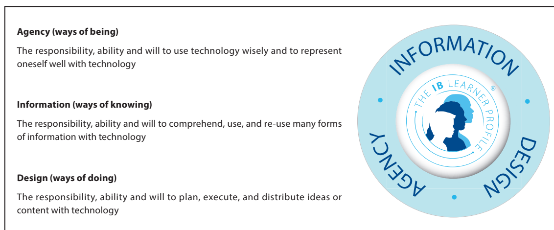
Figure 13 AID framework
