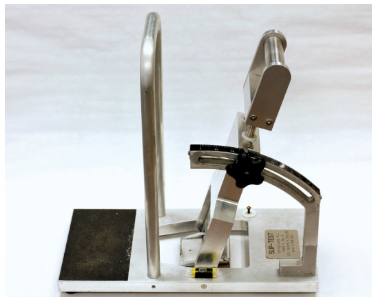
Figure 5: Brungraber Mark III 8
