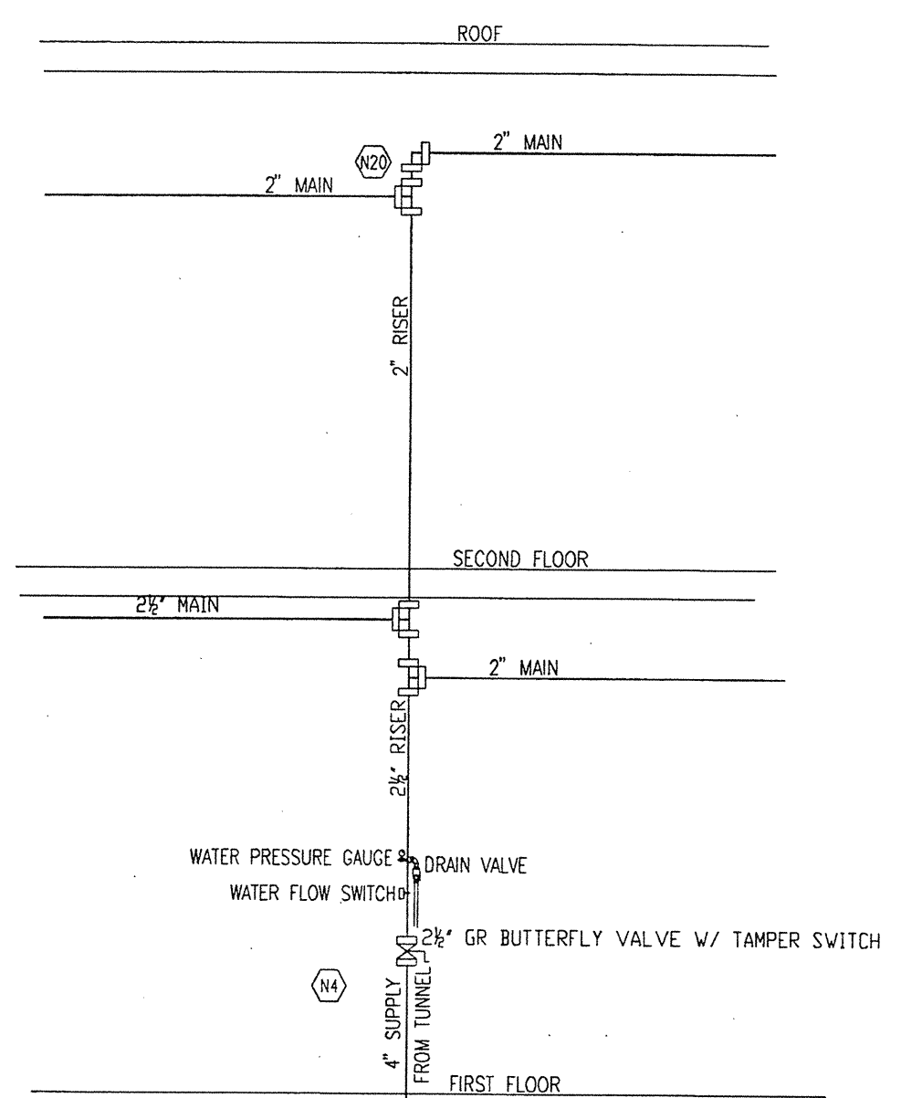
ZONE 1 RISER DETAIL
