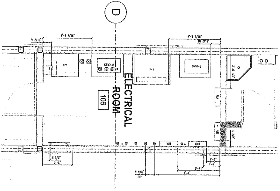
LEVEL 1 ELECTRICAL ROOM 106 LAYOUT
