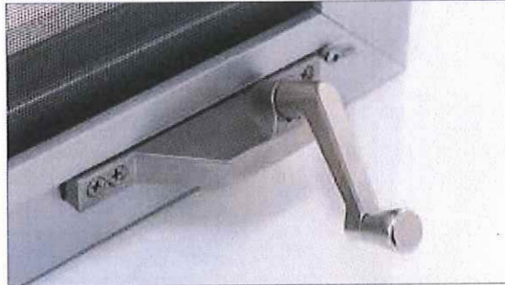
Left or Right Handed Roto Operator (Casement)
