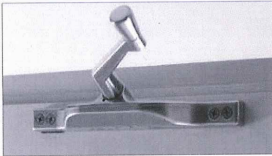
Pivot Shoe Roto Operator (Awning)
