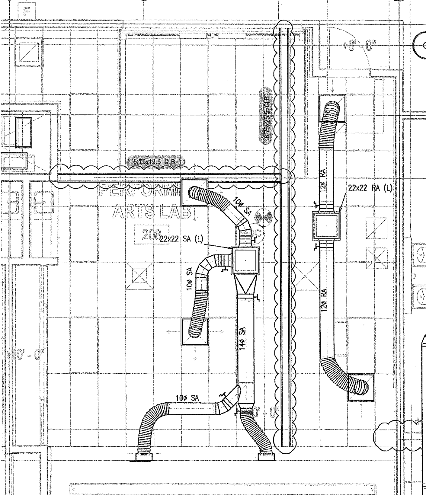
PERFORMING ARTS LAB 208 DUCT REDESIGN FOR LOW BEAMS
