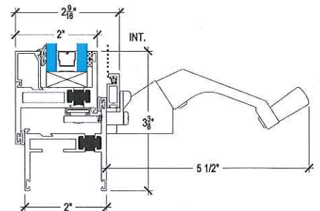
SILL
