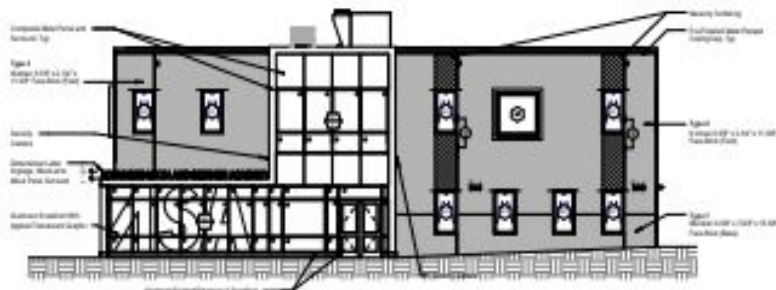
EAST ELEVATION
