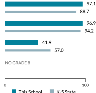
Area Scores
