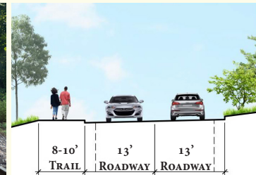
TYPICAL TRAIL SECTION ADJACENT TO ROADWAY
