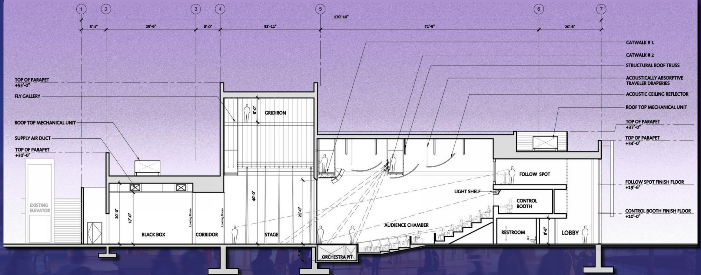
Building Section A
