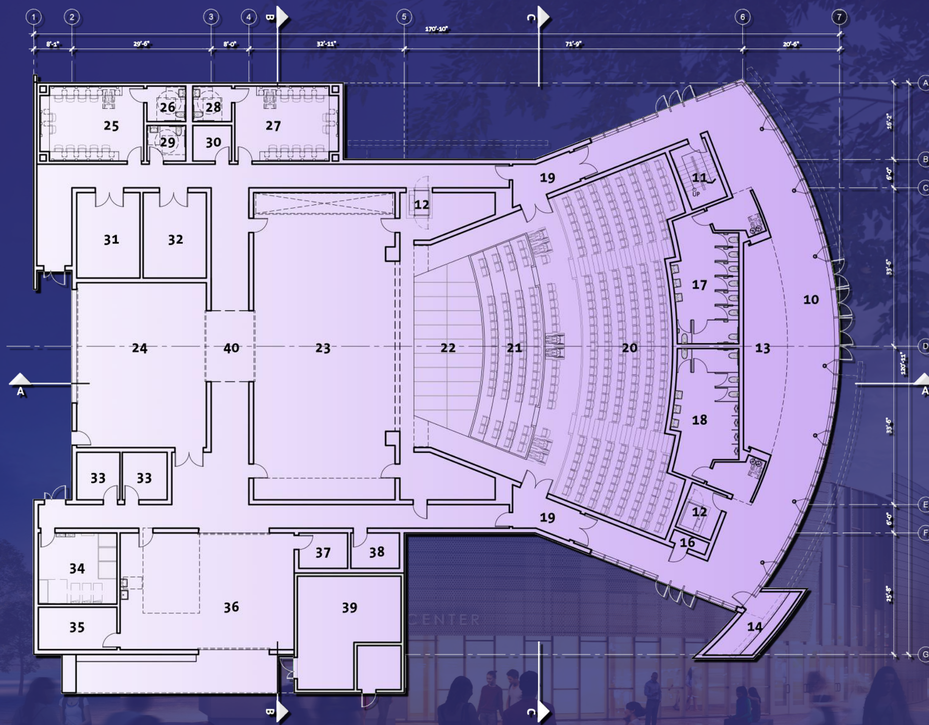
Orchestra Level Floor Plan
