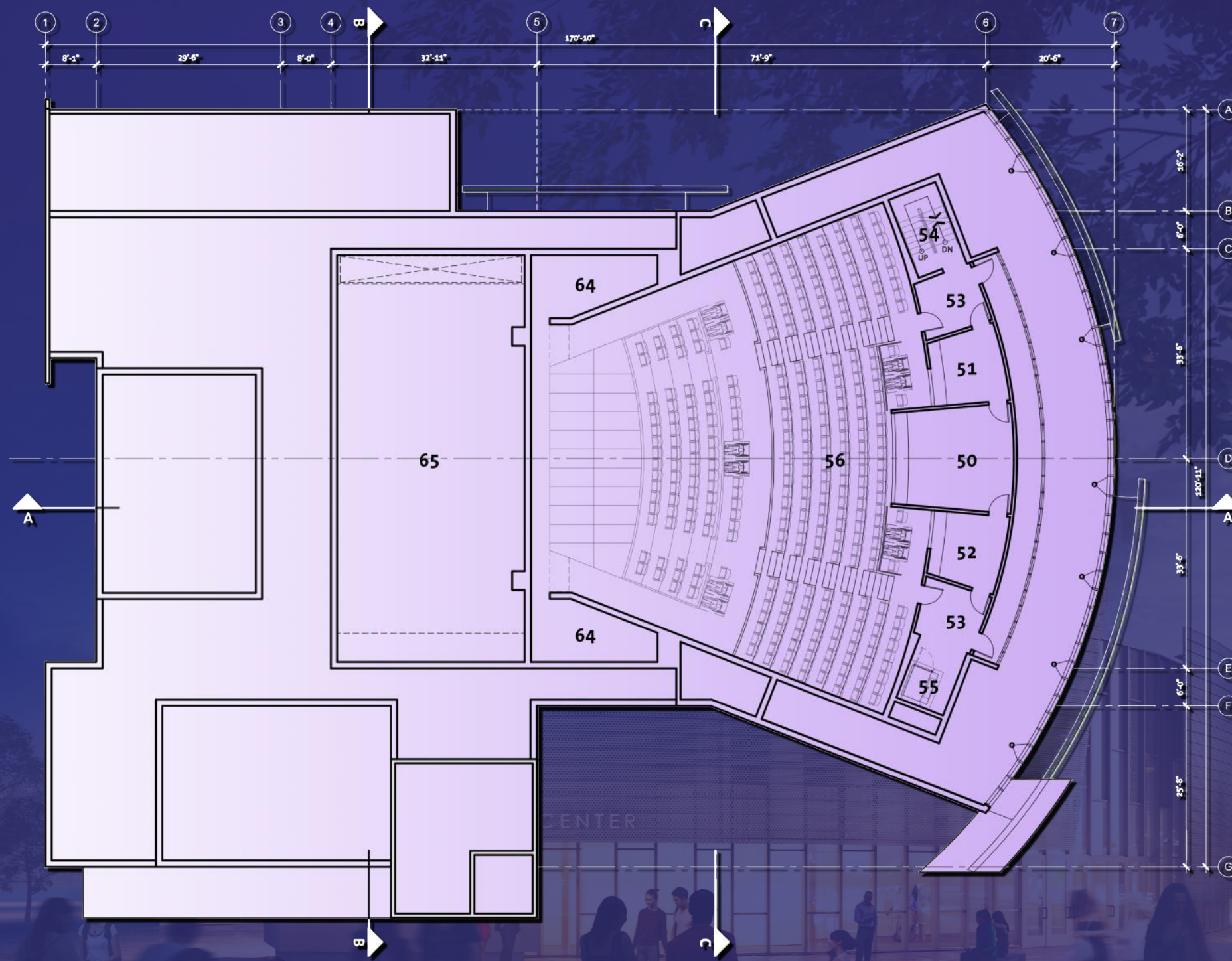
Parterre Level Floor Plan
