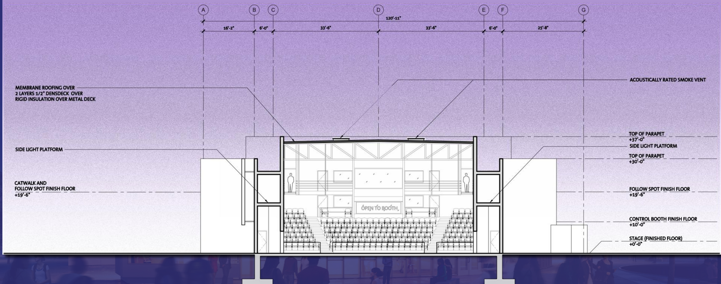
Building Section C
