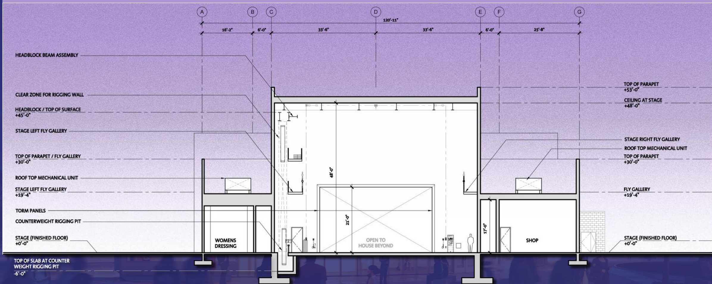
Building Section B
