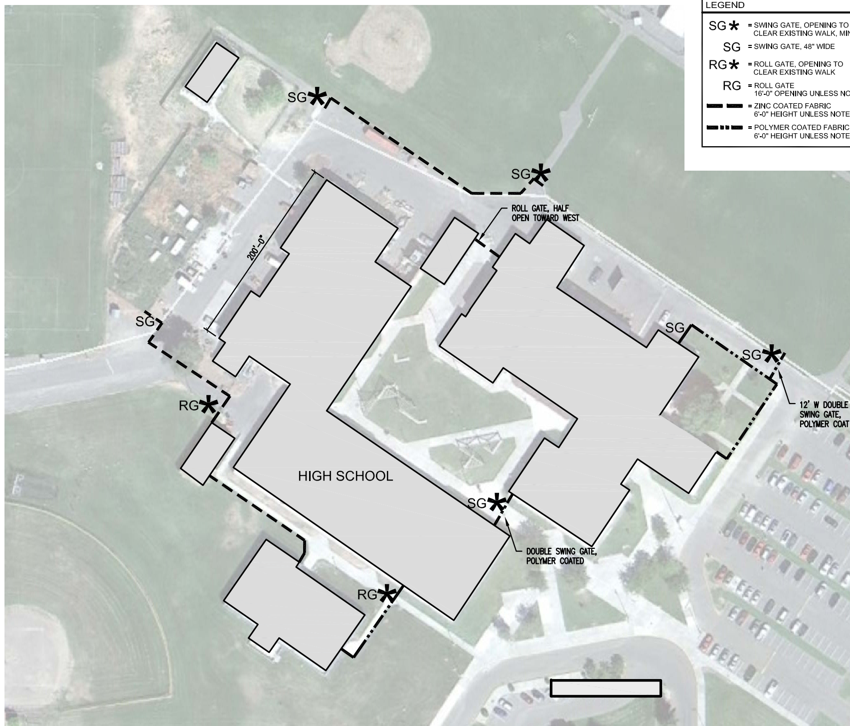
GRANDVIEW HIGH SCHOOL FENCING SITE PLAN
