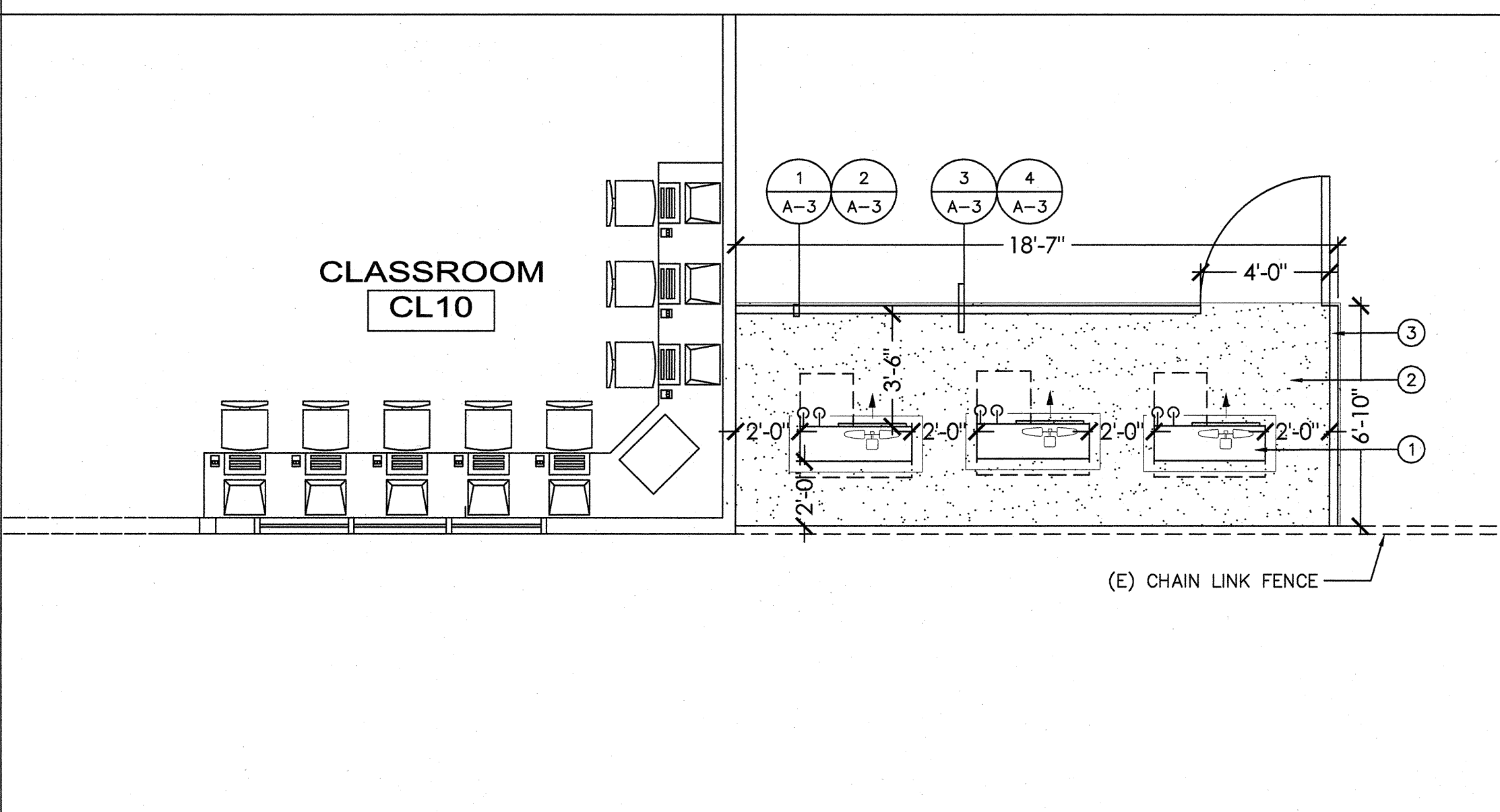
BUILDING 5 REMODEL FLOOR PLAN
