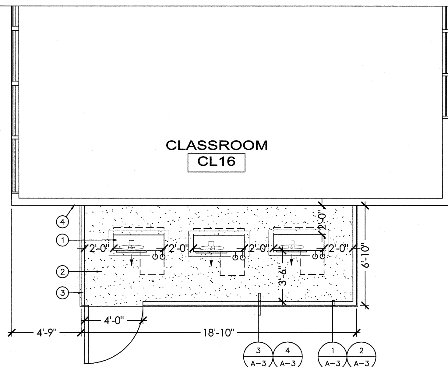
BUILDING 1 REMODEL FLOOR PLAN
