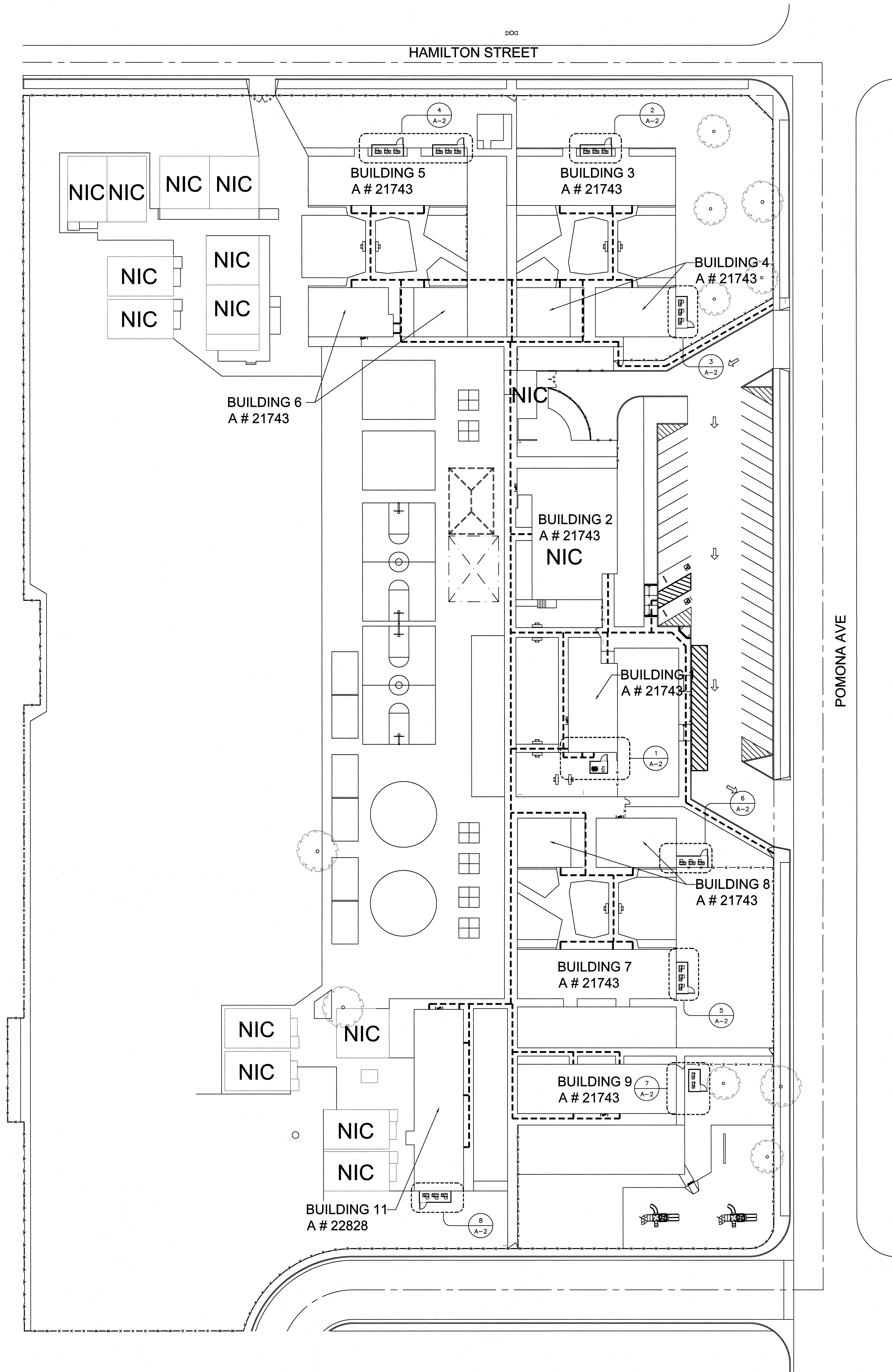
FENCE ENCLOSURE SITE PLAN
