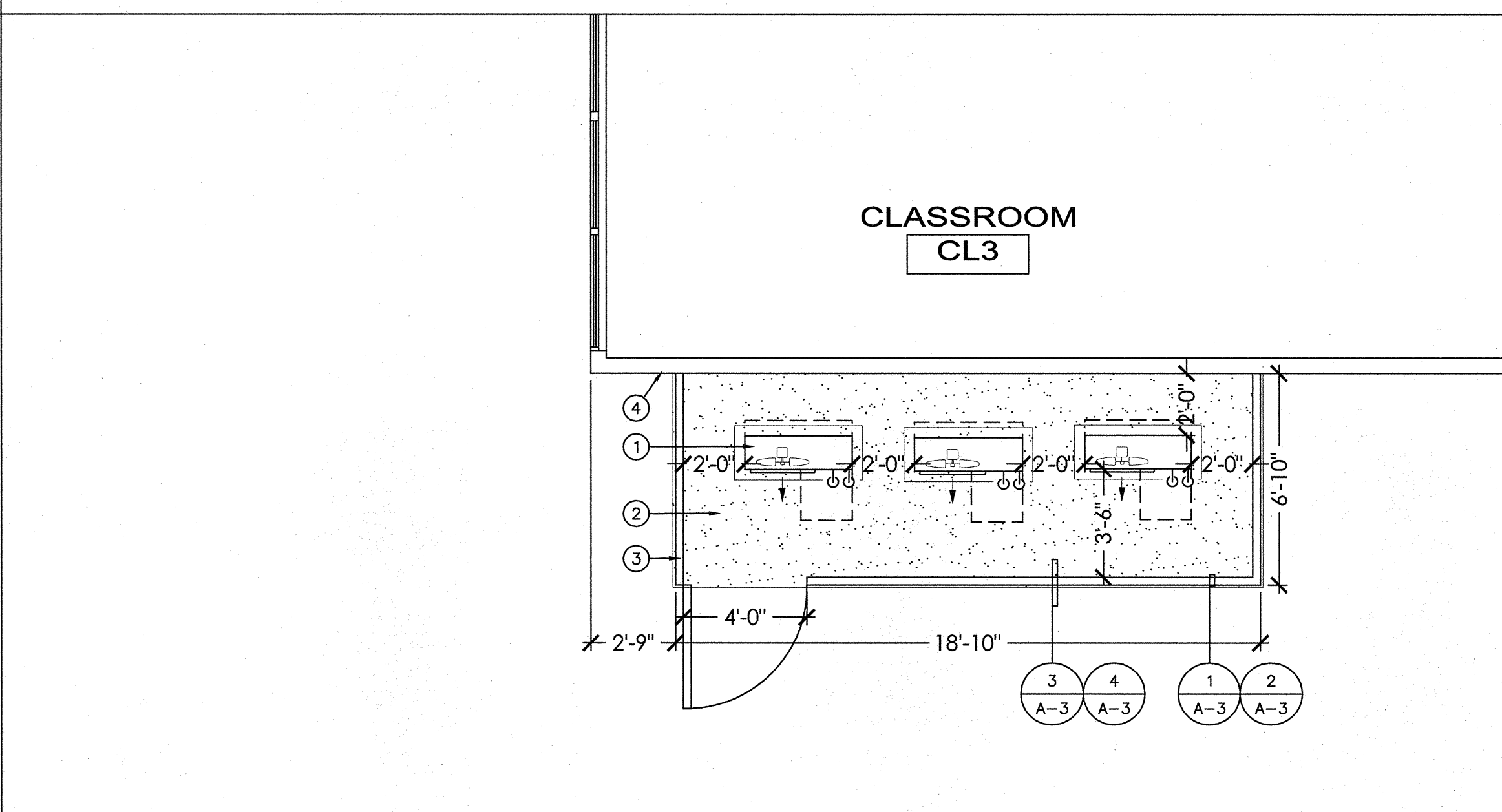
BUILDING 11 REMODEL FLOOR PLAN
