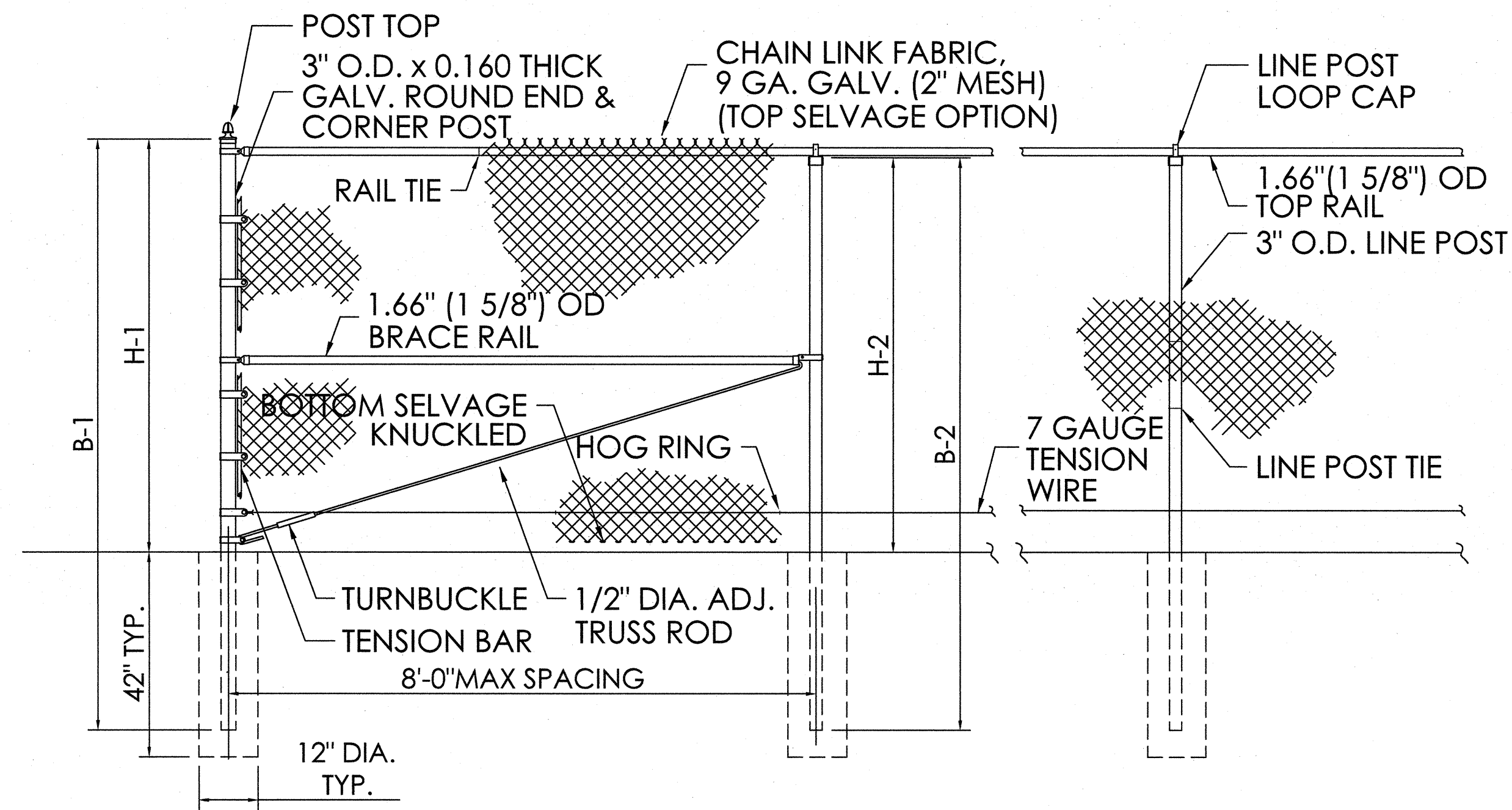
FENCE SECTION ELEVATION - ROUND END POSTS
