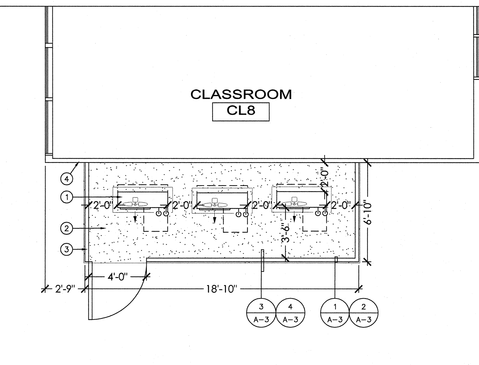
BUILDING 4 REMODEL FLOOR PLAN
