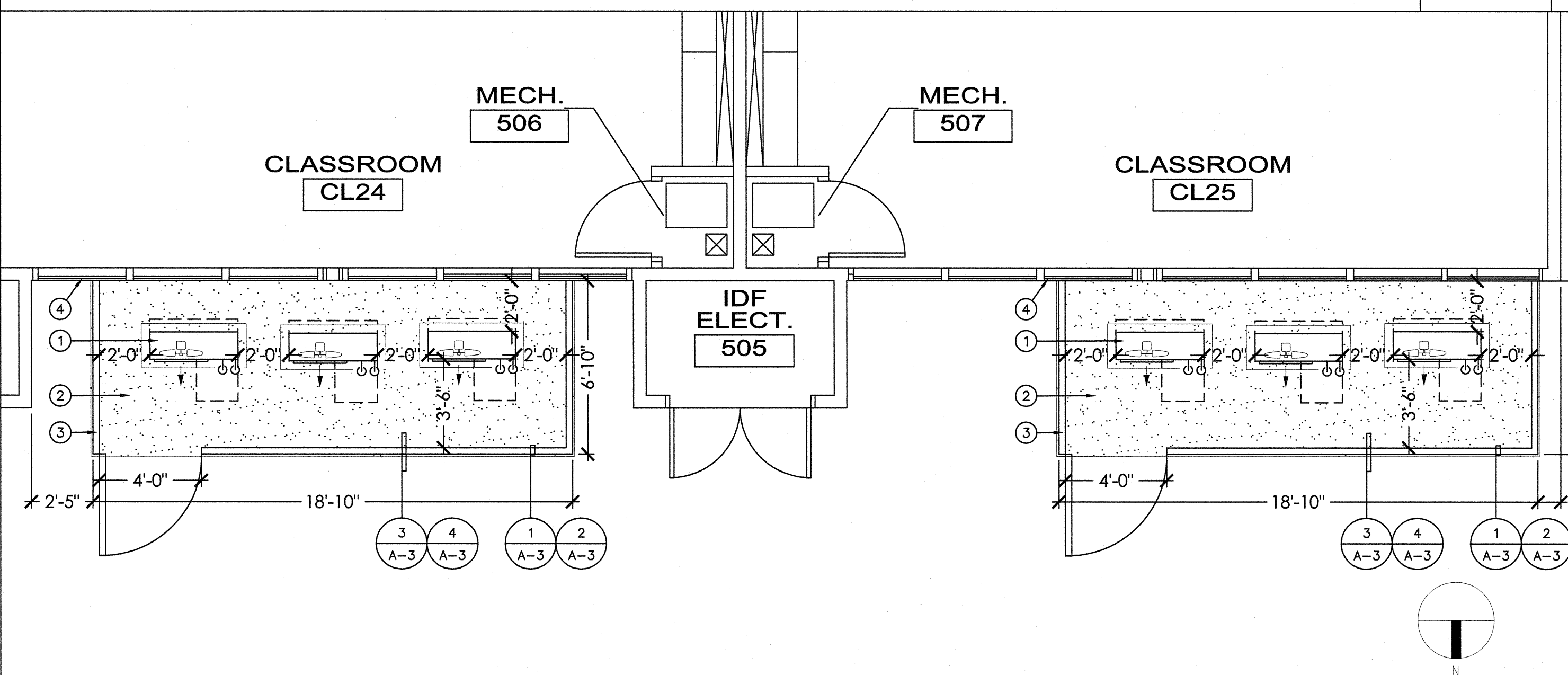
BUILDING 5 REMODEL FLOOR PLAN
