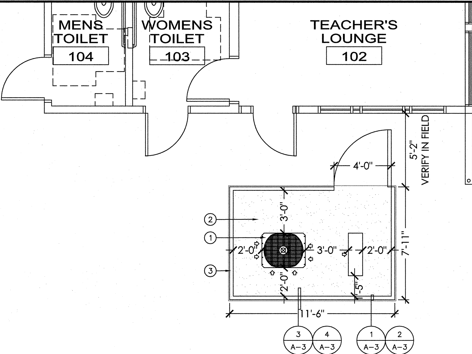
BUILDING 1 REMODEL FLOOR PLAN
