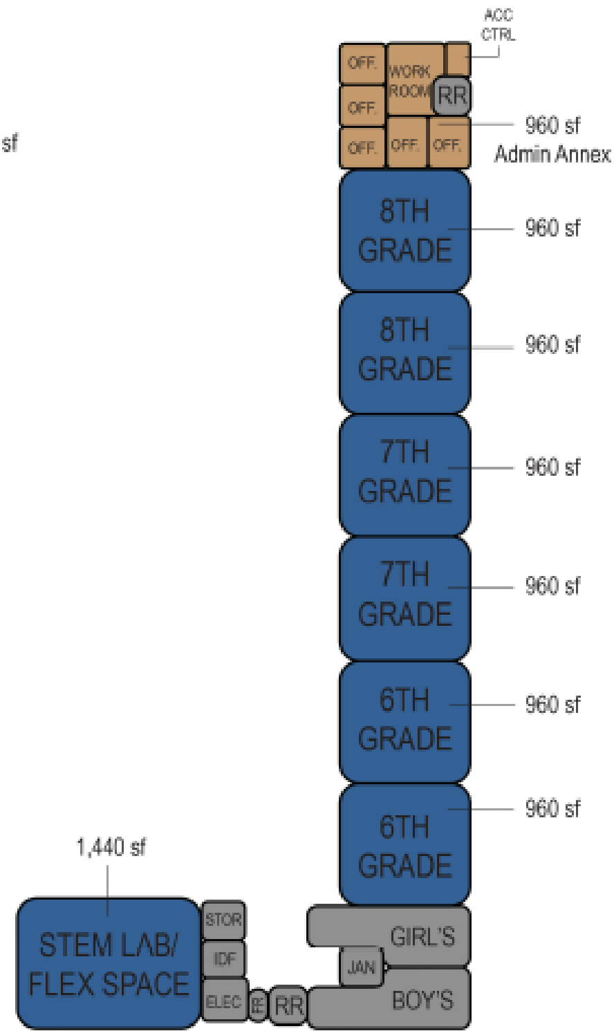
FLOOR PLAN / SINGLE STORY CLASSROOM BLDG.
