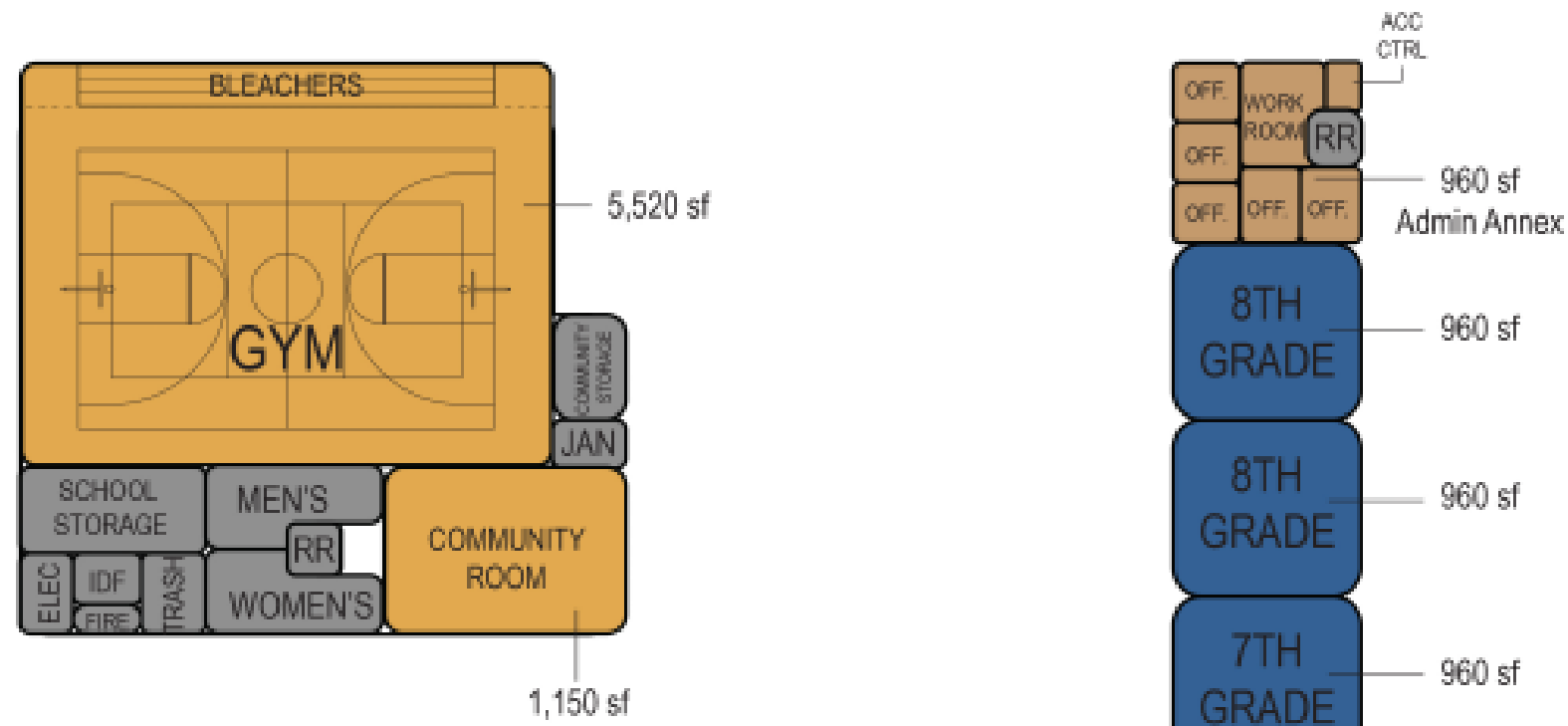
FLOOR PLAN / GYMNASIUM BLDG
