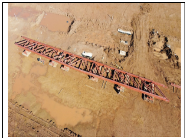
Girder Fabrication/Assembly
