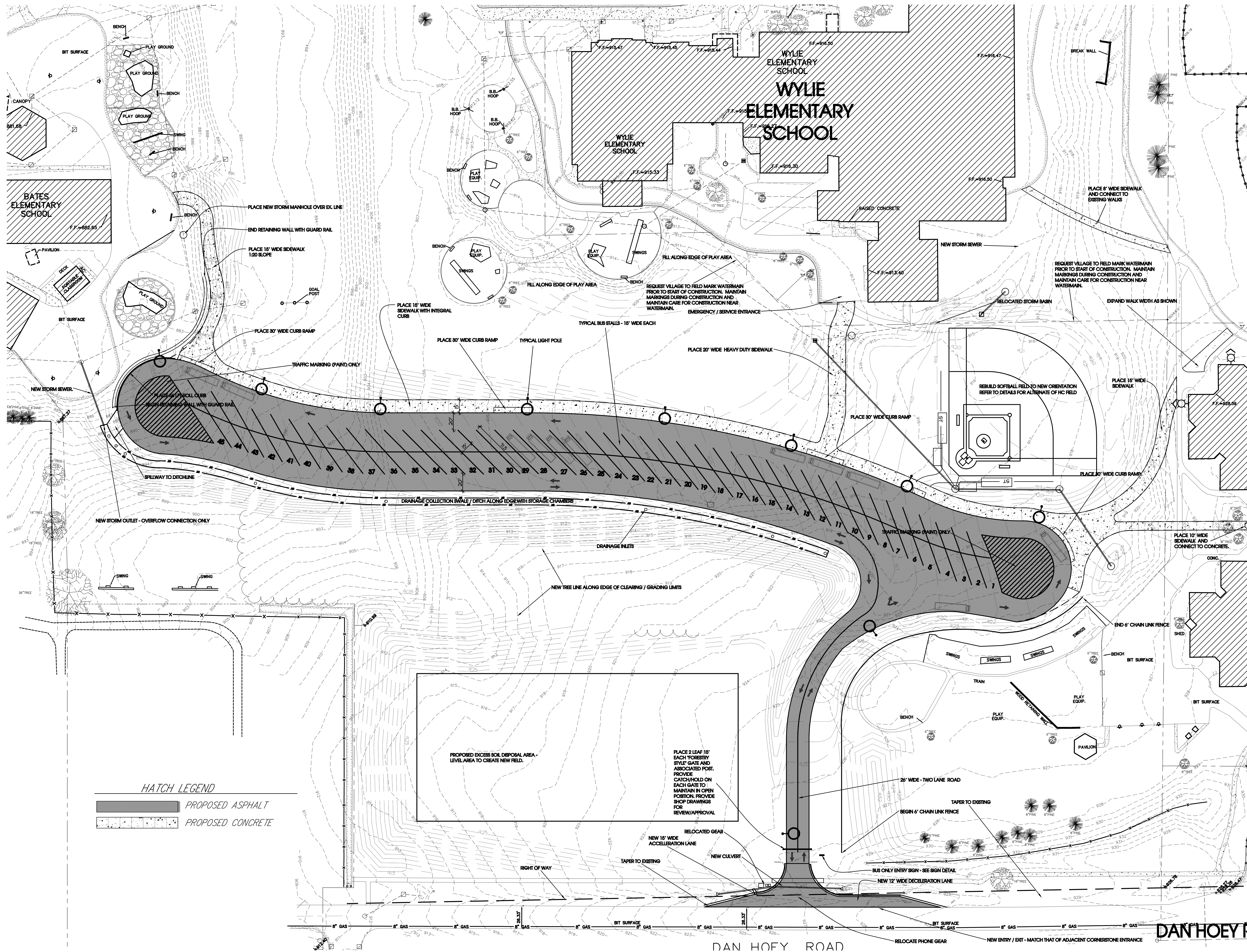
SITE IMPROVEMENTS PLAN SCALE 1" = 40'
