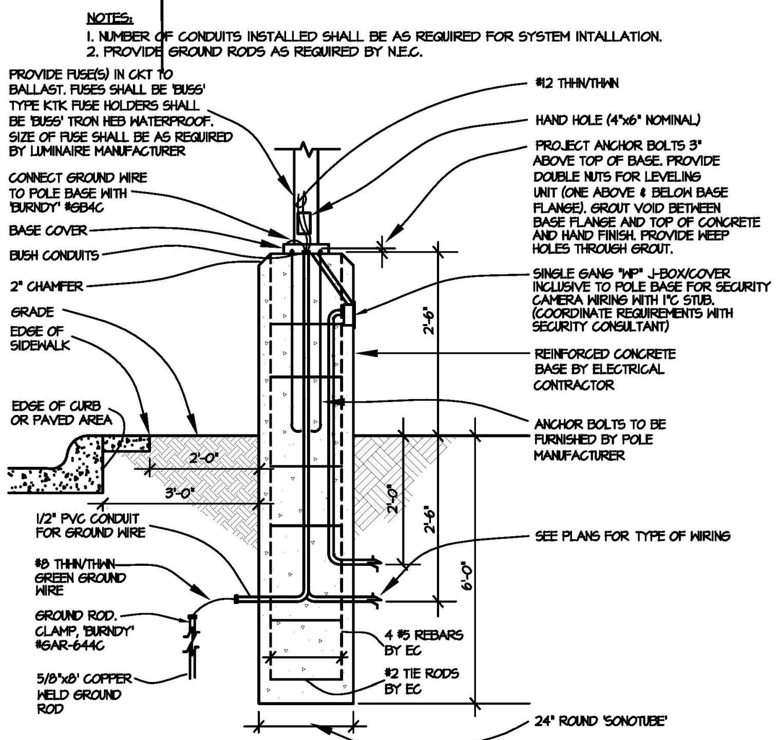
2 RAISED POLE BASE DETAIL NOT TO SCALE (TYPE SA)
