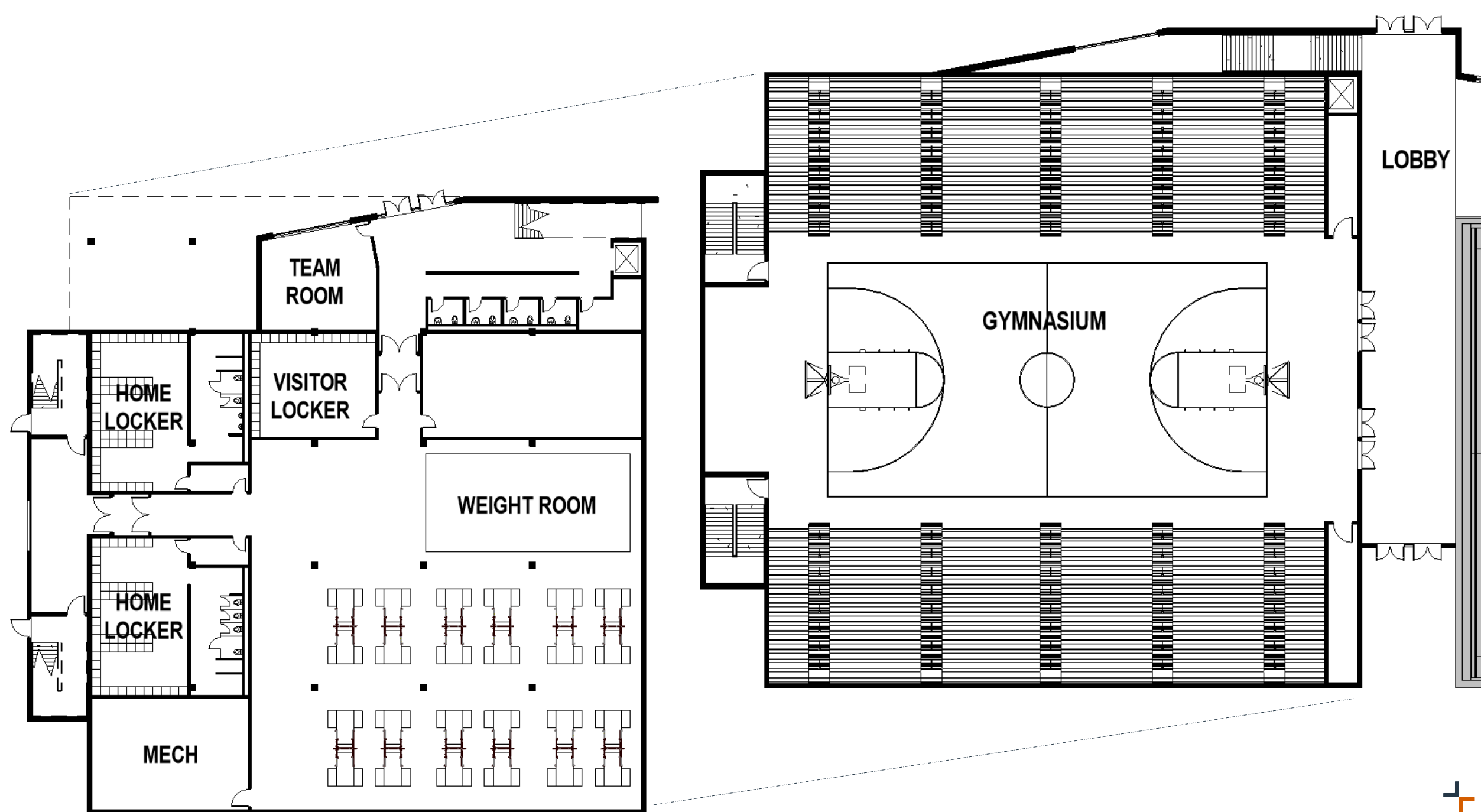
Lower Level
