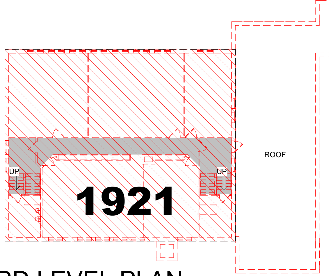
3 THIRD LEVEL PLAN 1/16" = 1'-0" 3,630 SF
