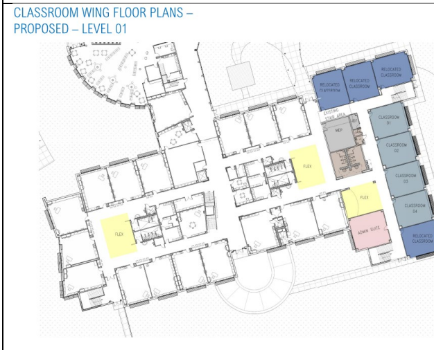
Proposed floor plans of classroom addition.
