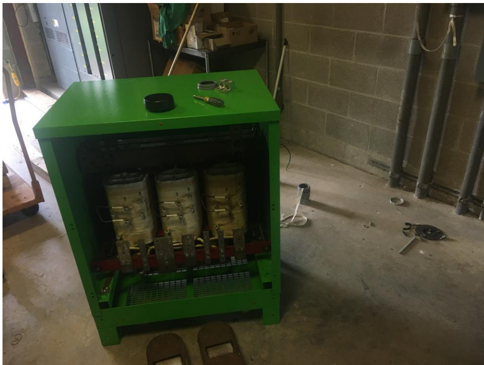
View of new transformer being installed in BES main Switchgear room.
