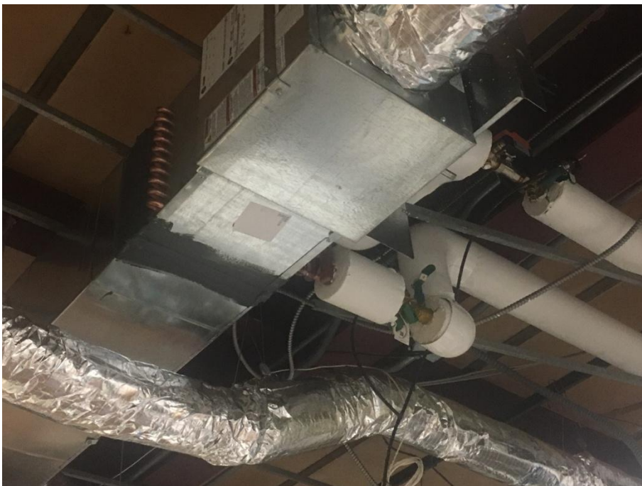
View of new VAV box with reheat coil.
