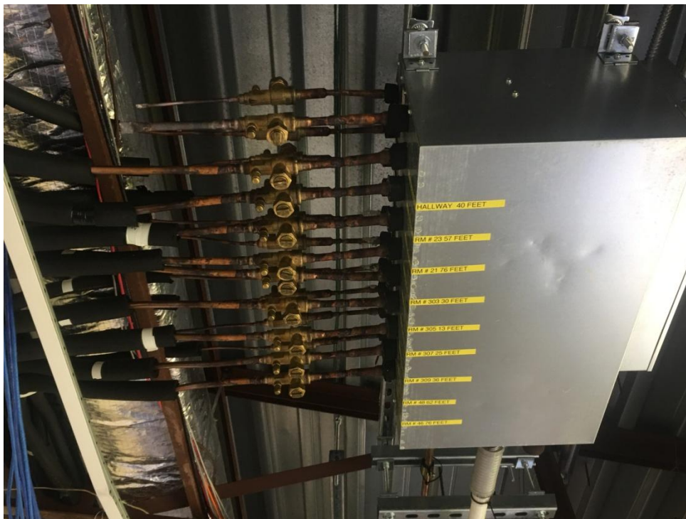
View of the Branch Controller #2 for Variable Refrigerant Volume system at BES.
