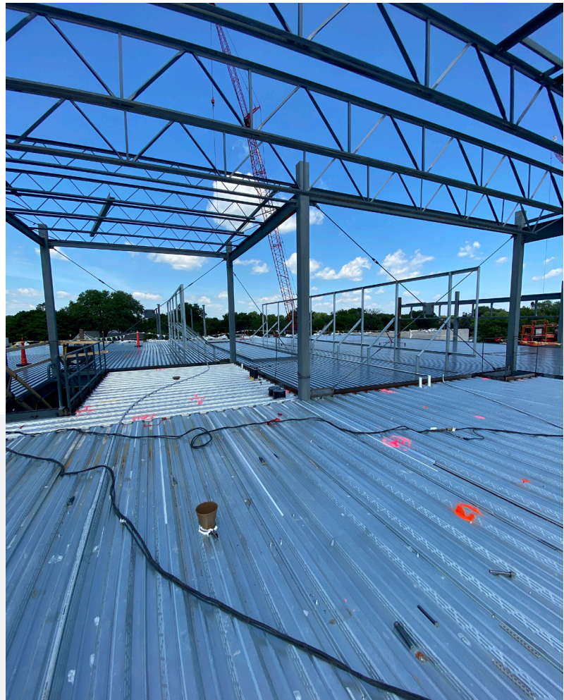
VEL PHILLIPS MIDDLE SCHOOL PENTHOUSE FOR HVAC
