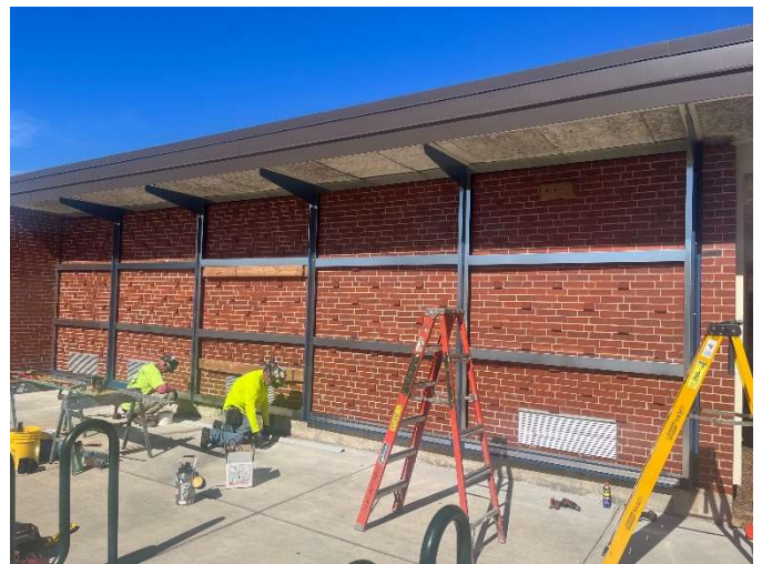
Metal wall panel installation on South Exterior
