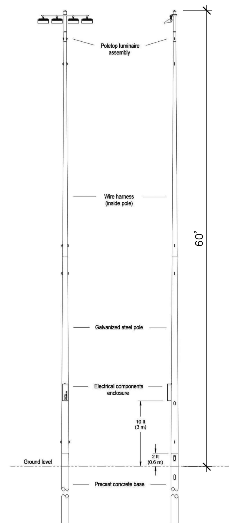
POLE HEIGHT AND FIXTURE COUNT VARIES, SEE TABLES THIS SHEET TYPICAL SPORTS LIGHT POLE SCALE: N.T.S.
