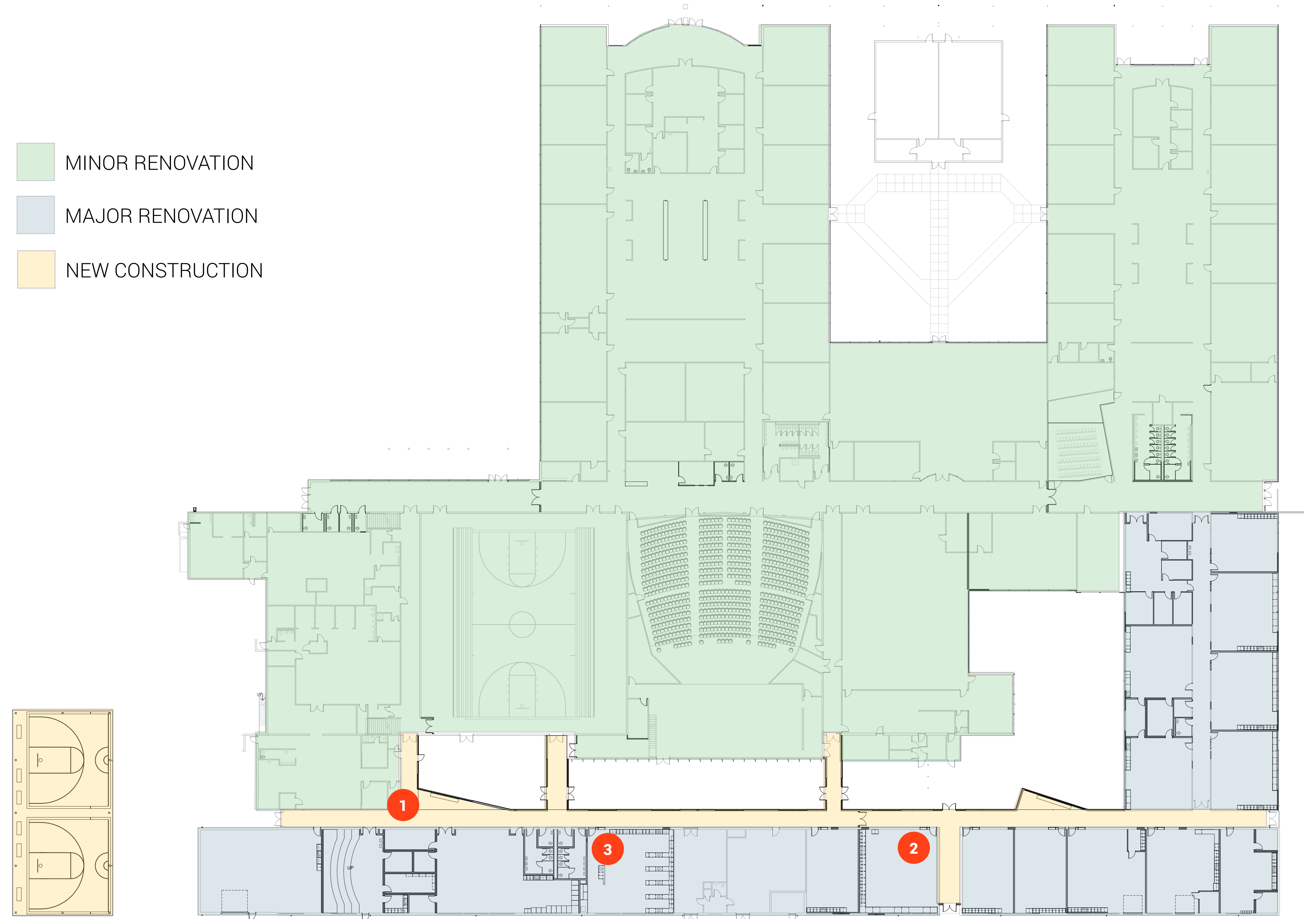
N ALDER CREEK MIDDLE SCHOOL - FLOOR PLAN
