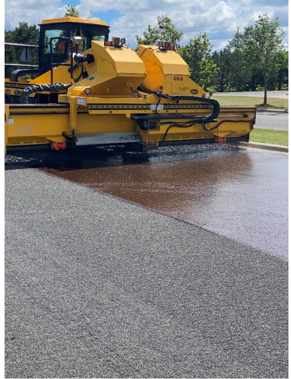
"chip" rocks being applied on top of seal coat to finish 1 st layer of new surfacing
