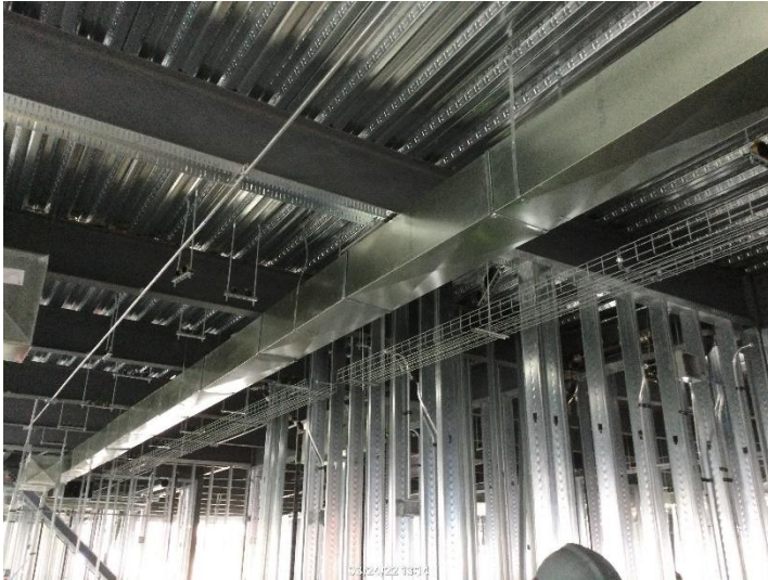
Overhead Ductwork and Cable Tray Installation
