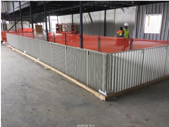
Area B handrail installation
