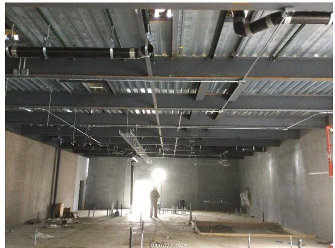
Electrical and HVAC hangers installed in kitchen
