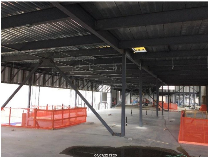
Electrical and HVAC hangers installation in Area A
