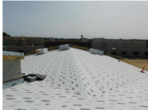
Unit B roof dry in
