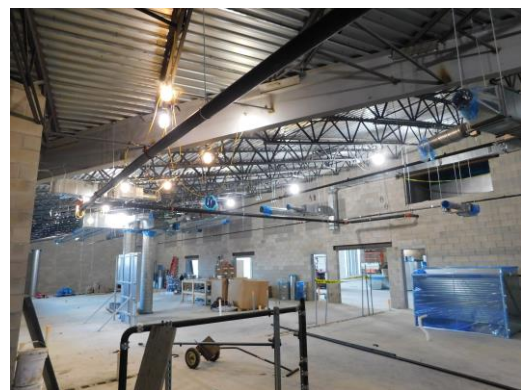
Fire suppression piping being installed in the kitchen area
