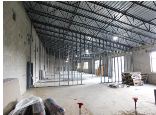
Metal studs being installed in the 2 nd floor classroom wing area
