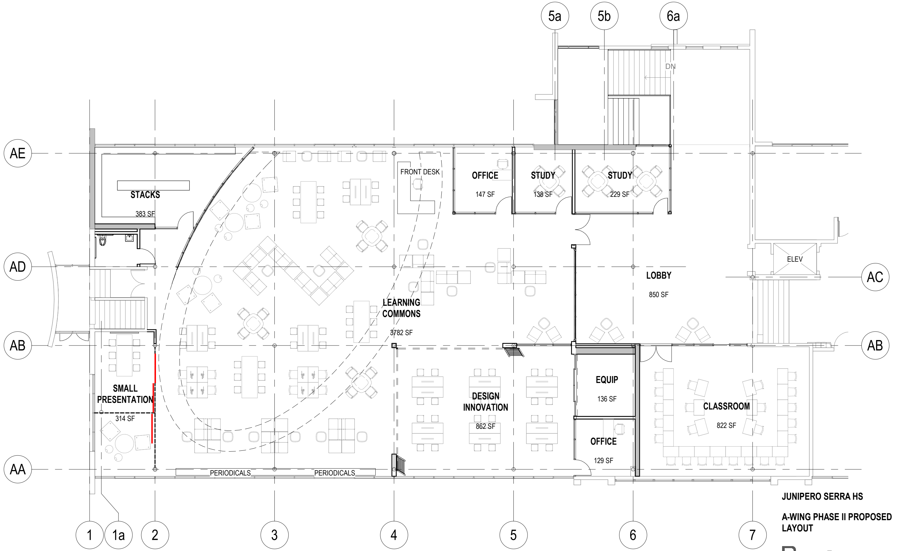
1 2ND FLOOR PLAN 3/32" = 1'-0"
