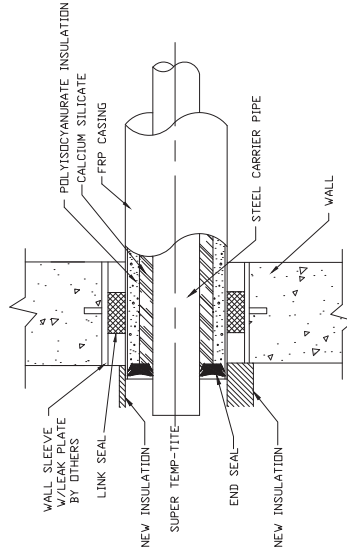
WALL PENETRATION DETAILS NO SCALE
