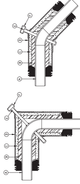
SUPER TEMP-TITE JOINT CROSS SECTION NO SCALE
