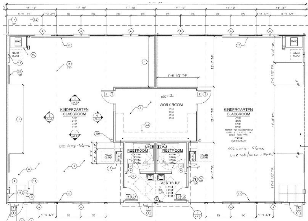
Figure 1 – Sample Kindergarten Floor Plan
