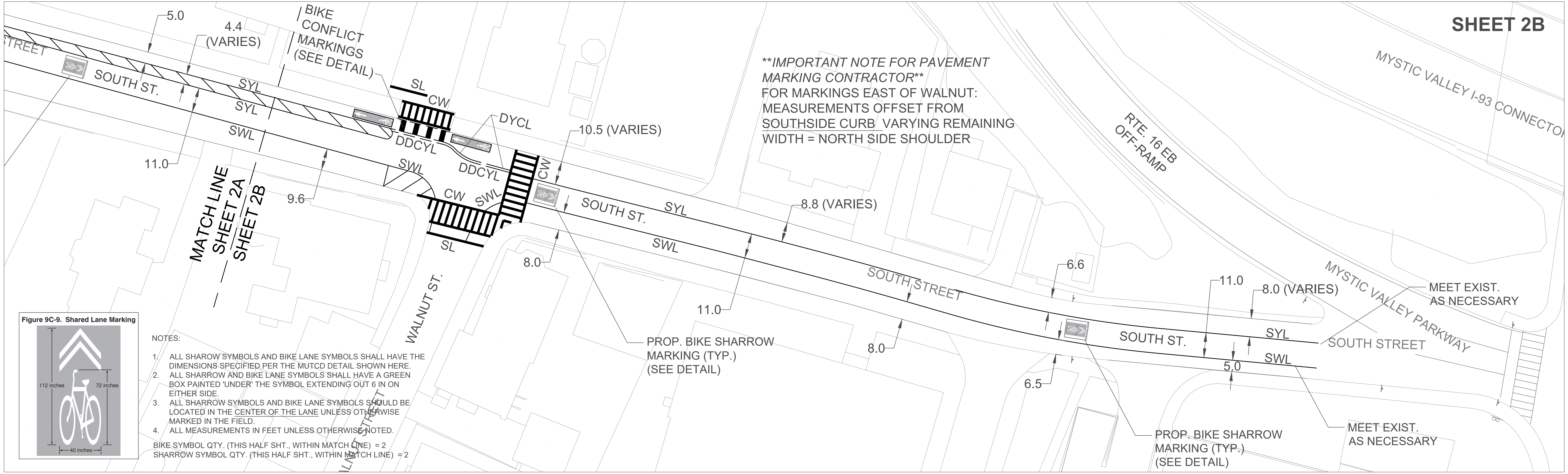
Figure 9C-9. Shared Lane Marking
