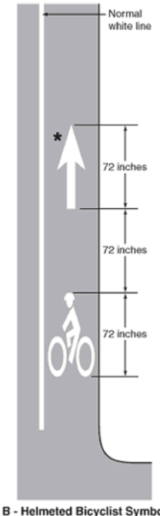
B - Helmeted Bicyclist Symbol
