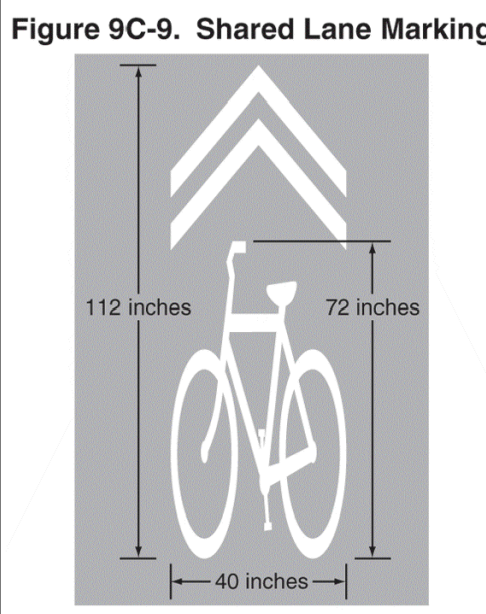
Figure 9C-9. Shared Lane Marking
