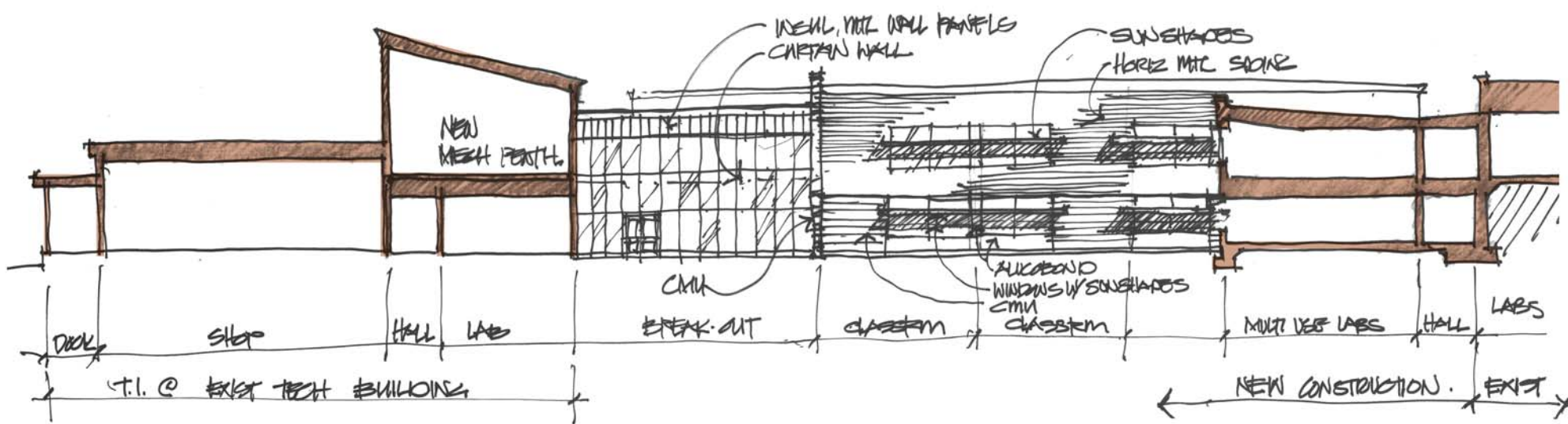
D SECTION / COURT NORTH FACADE
