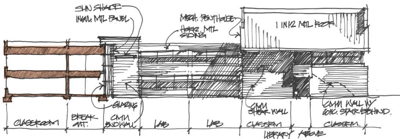
E SECTION / EAST FACADE
