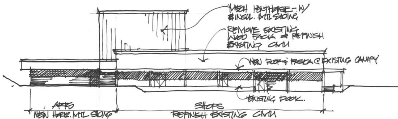
F TECH BUILDING WEST FACADE
