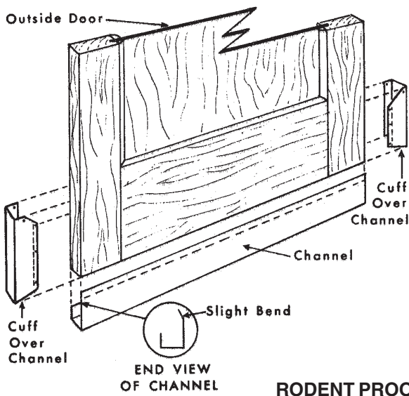
RODENT PROOFING OF A DOOR
