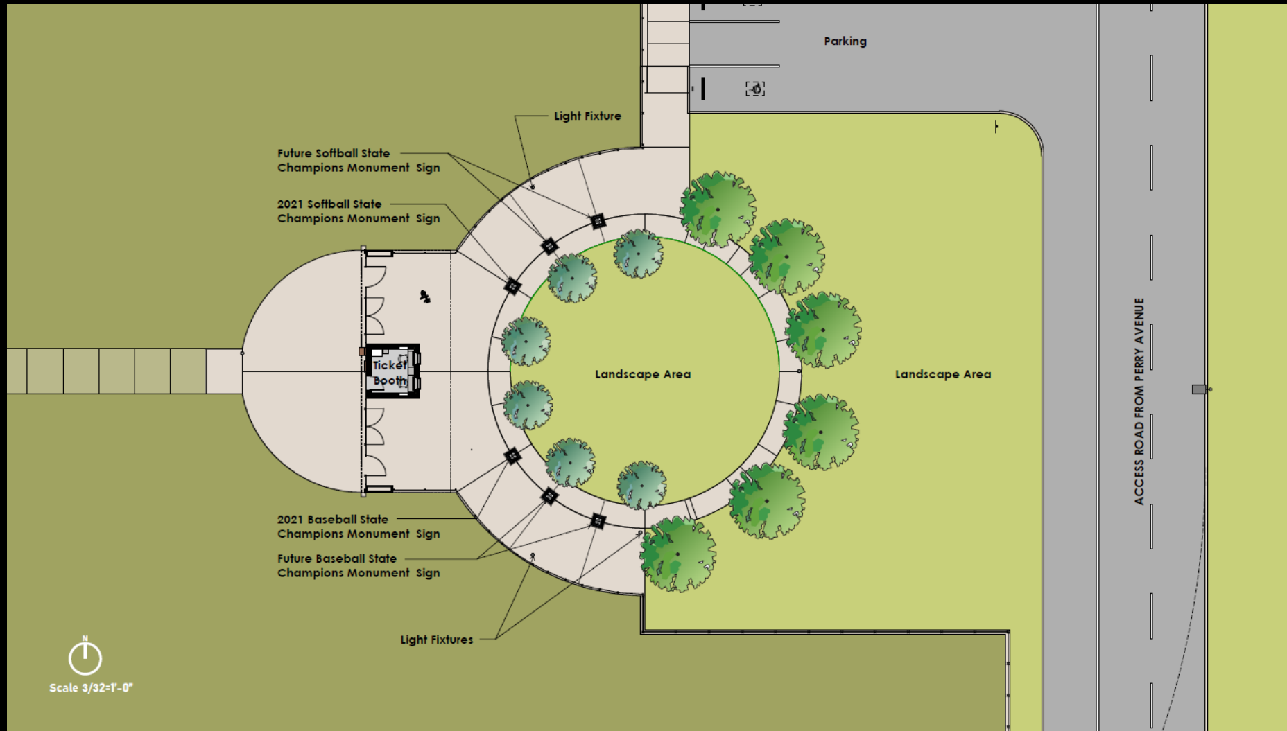
BARBERS HILL ISD STATE CHAMPIONSHIP MONUMENT SIGN - SITE PLAN
