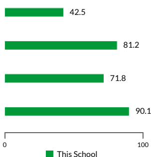
Group Scores
