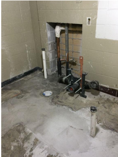
Toilet 121 Rough-in
