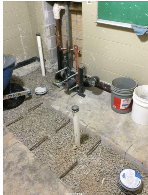
Underground Rough-in Toilet 121
