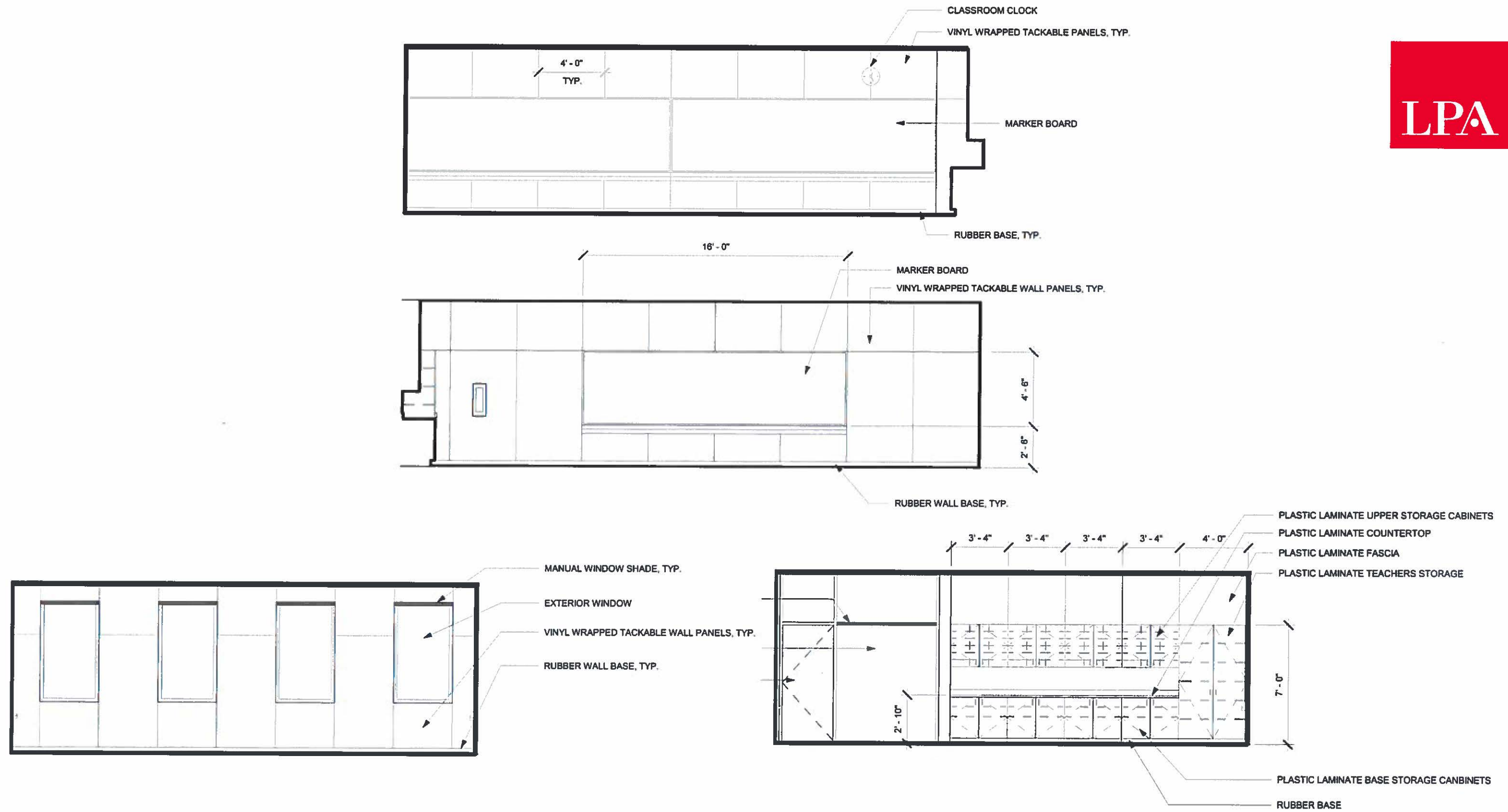
typical classroom – interior elevations
