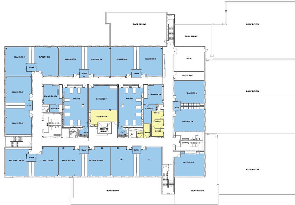
COMPOSITE THIRD FLOOR PLAN 1" = 30'-0"
