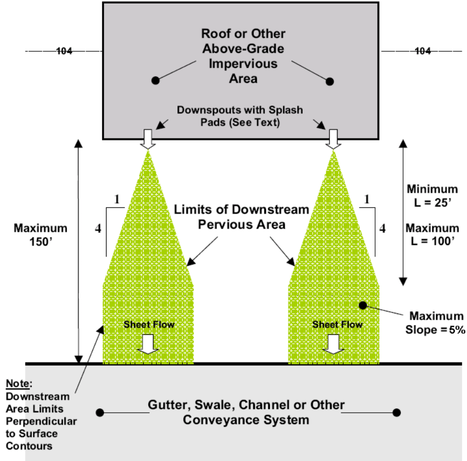
Figure 4.17 – Standards for disconnecting impervious surface via downsports. Source: New Jersey Department of Environmental Protection, 2004.
