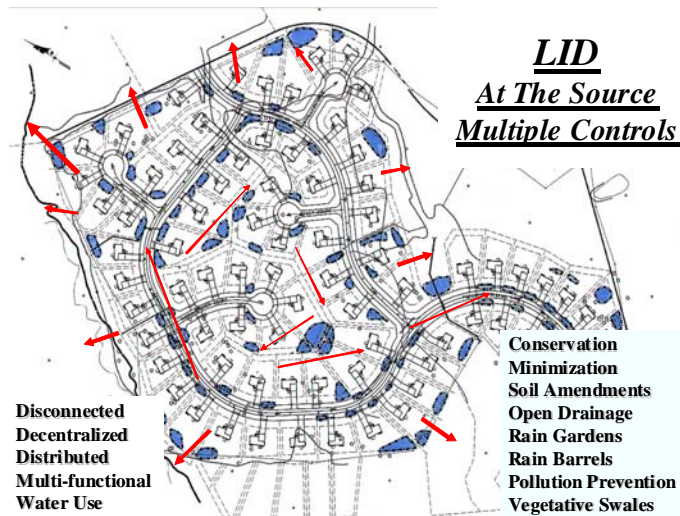
Figure 2.2 – LID Controls. A LID approach uses a wide array of techniques that work with the landscape, soils, drainage patterns and vegetation to minimize impacts and integrated management controls to retain, detain, infiltrate and filter runoff. LID can provide better stormwater controls by mimicking the pre-development hydrology. Often LID designs increase lot yield and reduce infrastructure cost.
