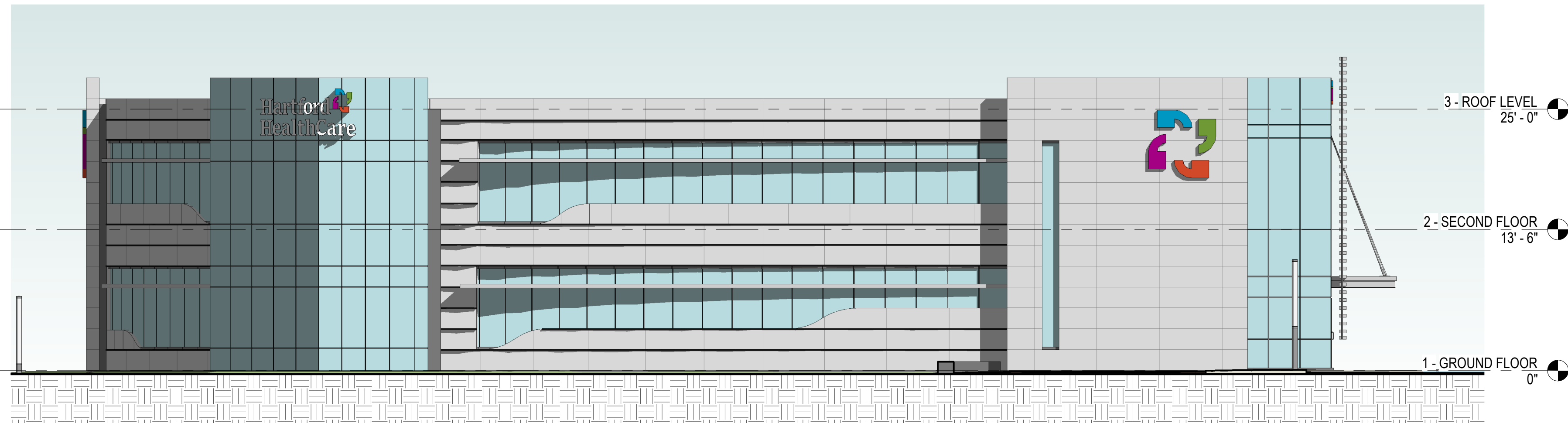
3 WEST ELEVATION PR6 1/8" = 1'-0"
