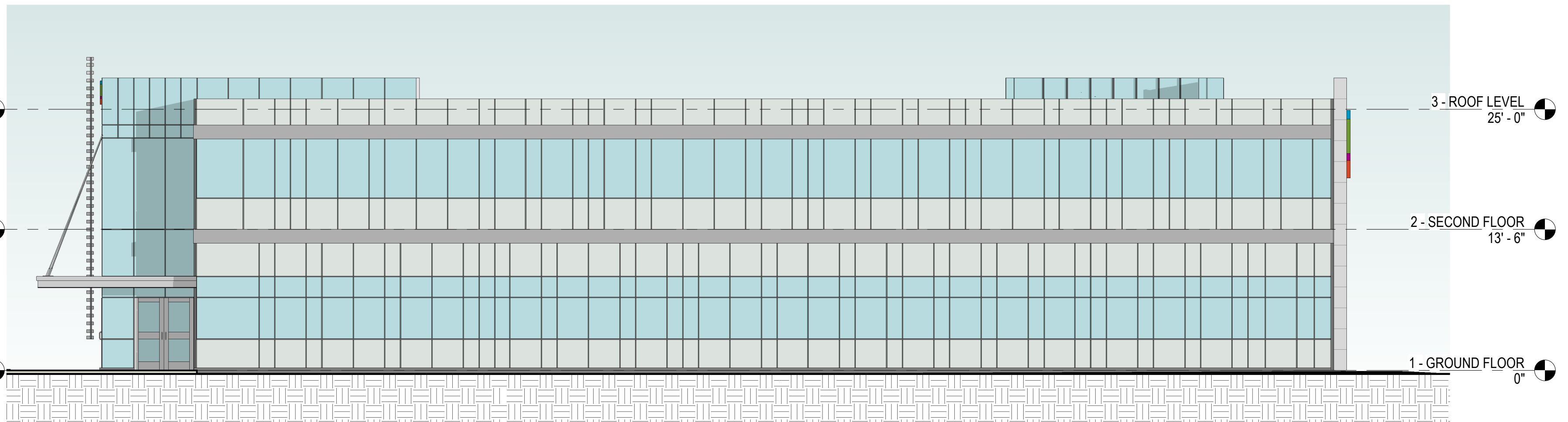
1 EAST ELEVATION PR6 1/8" = 1'-0"
