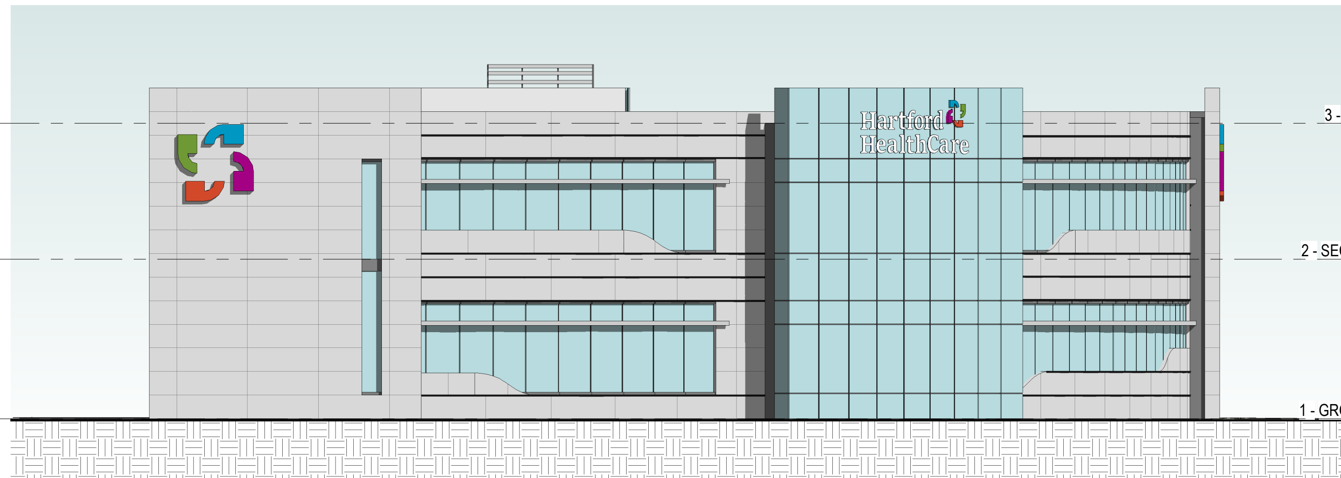
4 NORTH ELEVATION PR6 1/8" = 1'-0"
