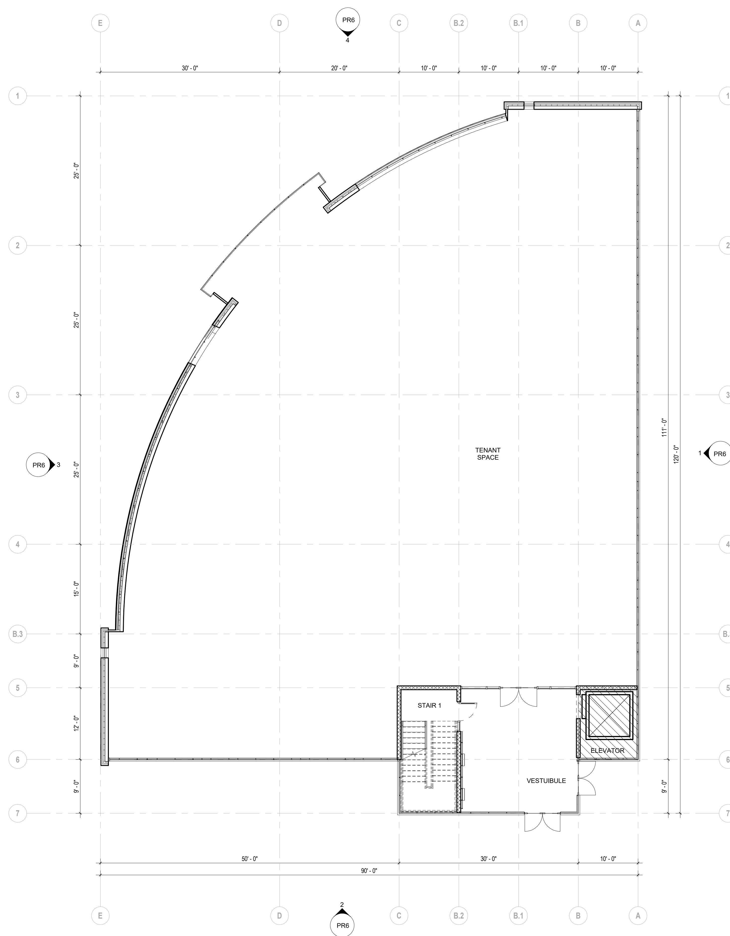
1 FIRST FLOOR PLAN PR5 1/8" = 1'-0"
