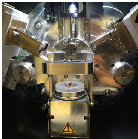
f) sample mounted for XRD test
