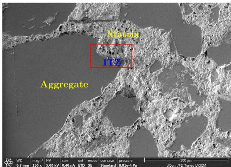
Fig. 7.1 Porous micro structure of matrix
