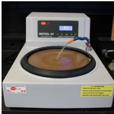
b) Rotary grinding and polishing machine
