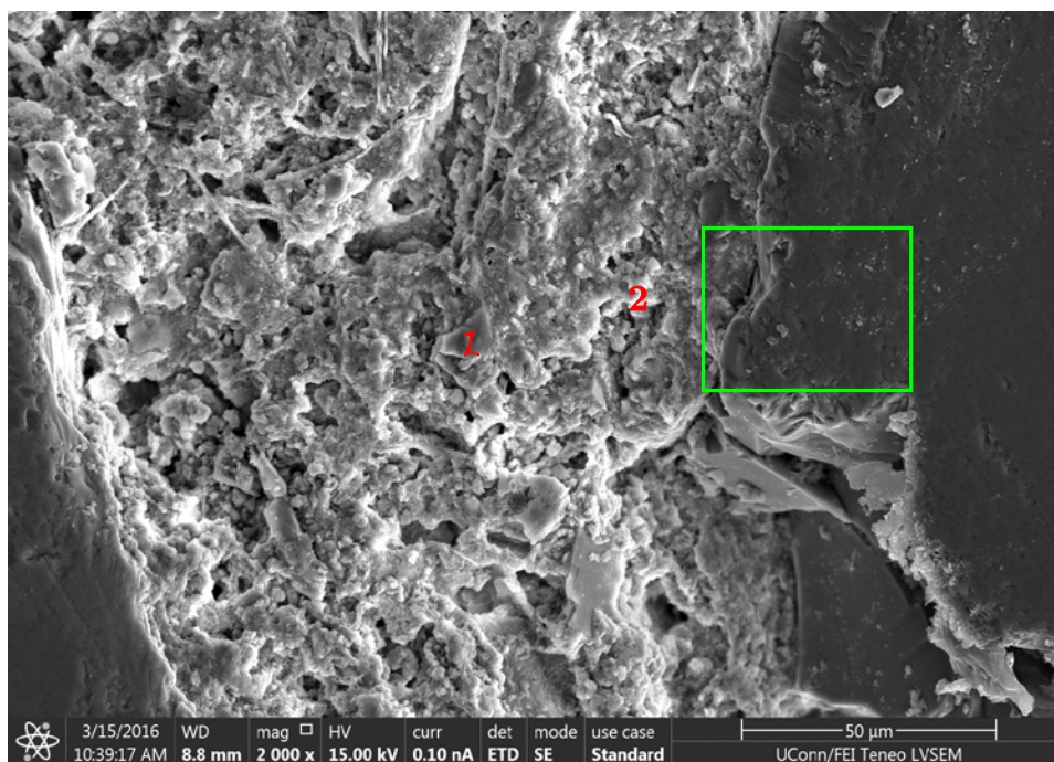
Fig. E- 1 Pyrrhotite-bearing aggregate
