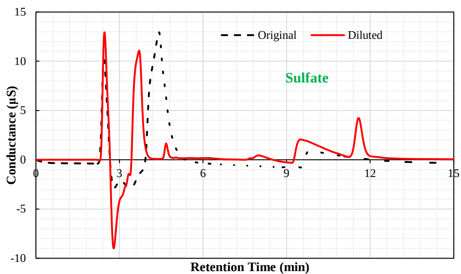
Fig. 5.8 Comparison of IC signal
