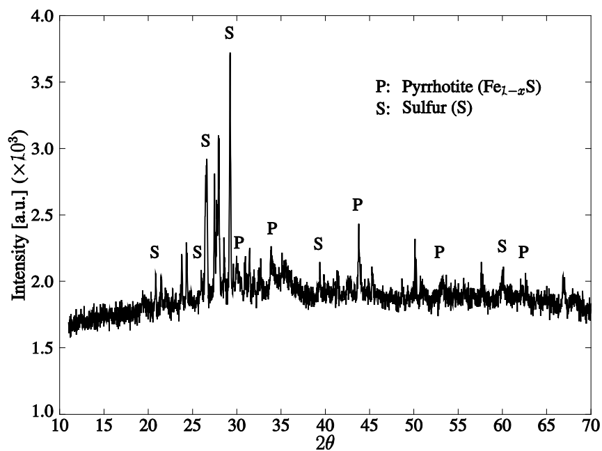
Fig. 6.4 XRD pattern of aggregate showing the oxidization product of sulfur
