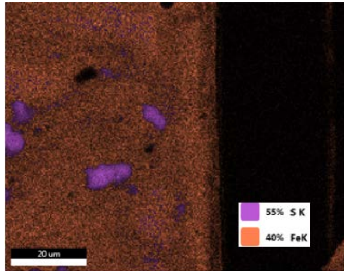
Fig. 5.14 EDX mapping elementary analysis for the interface zone - Sample 1
