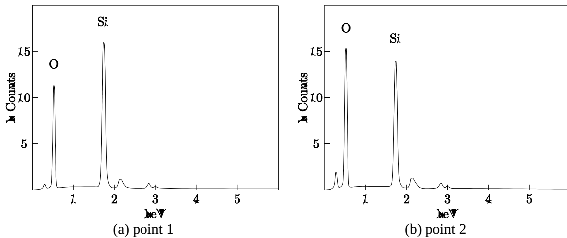
Fig. 7.14 EDX result for aggregate
