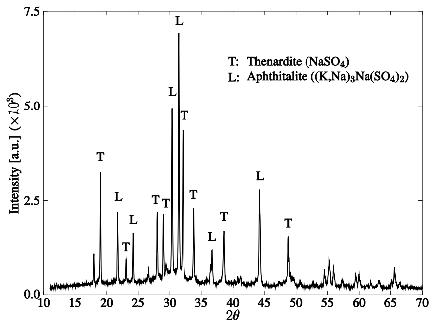
Fig. 6.7 Typical XRD pattern of whitish formation – housing 7
