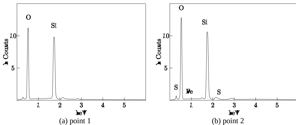
Fig. 7.9 EDS spectrum – aggregate
