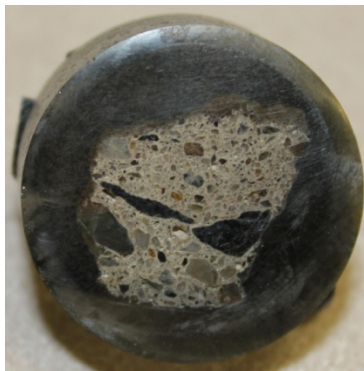
a) samples impregnated with low viscosity resin
