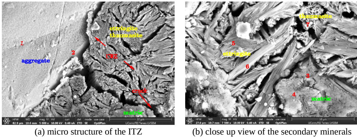
Fig. 7.8 Secondary minerals in the ITZ
