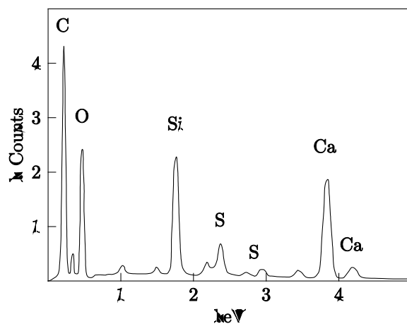
Fig. F- 4 EDS spectrum of point 3 matrix
