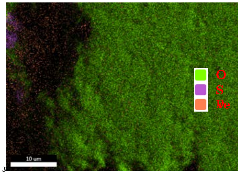
Fig. E- 4 EDS mapping analysis – Rectangular area in Fig. E- 1
