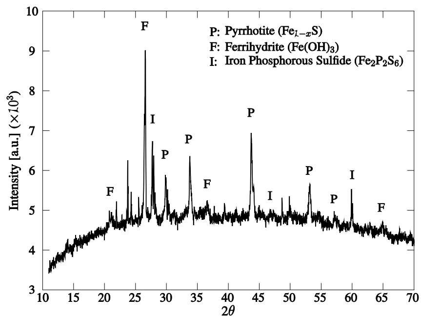
Fig. 6.3 XRD pattern of aggregate showing the oxidization product of ferrihydrite
