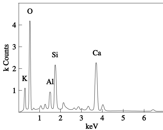
Fig. E- 3 DEX spectrum – point 2
