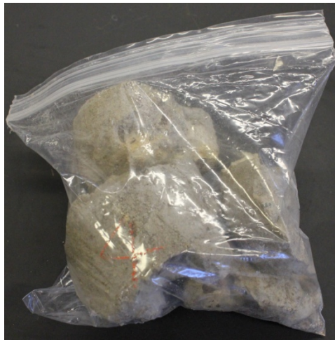
Fig. 4.4 Completely disintegrated core sample of concrete foundation wall– house 1
