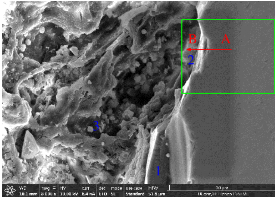
Fig. 7.2 Micro structure of the investigated ITZ
