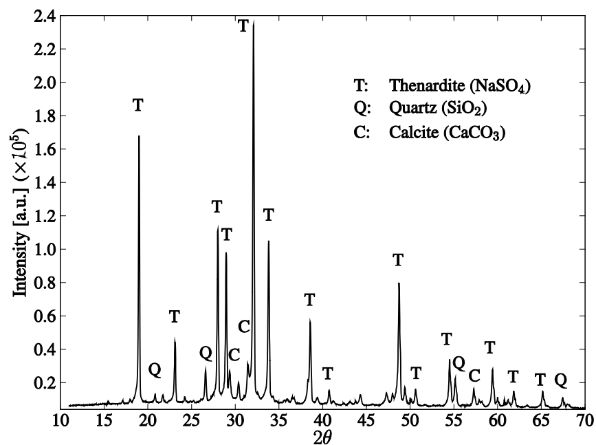
Fig. 6.6 Typical XRD pattern of whitish formation - housing 1
