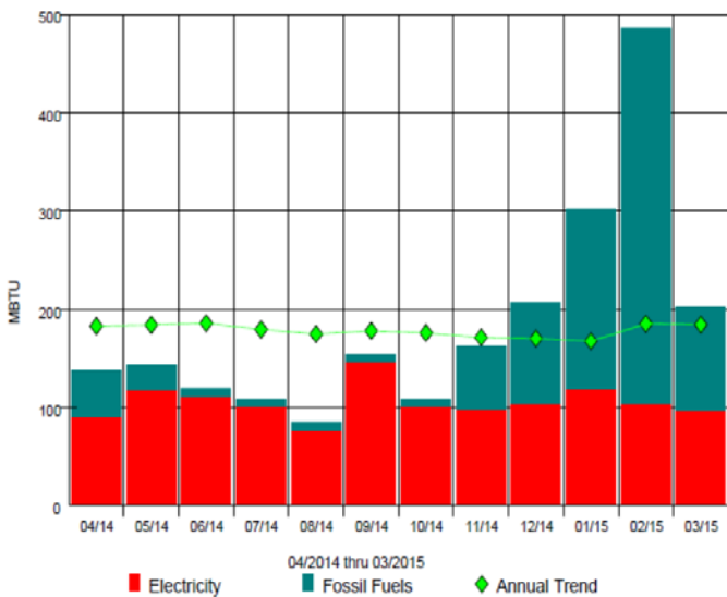
Energy Use Graph - Monthly and Annual Trend for Stony Point Elementary
