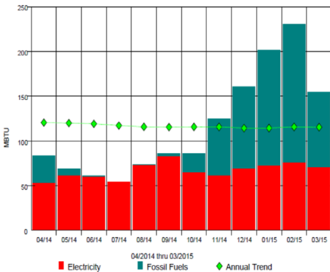
Energy Use Graph - Monthly and Annual Trend for Murray High
