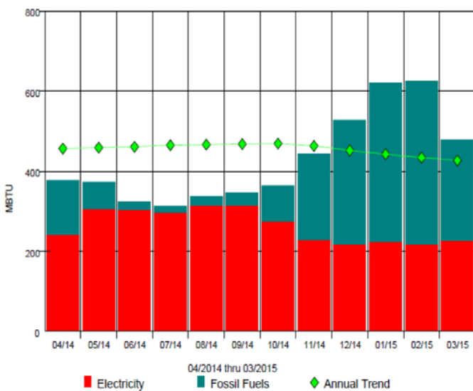
Energy Use Graph - Monthly and Annual Trend for Burley Middle
