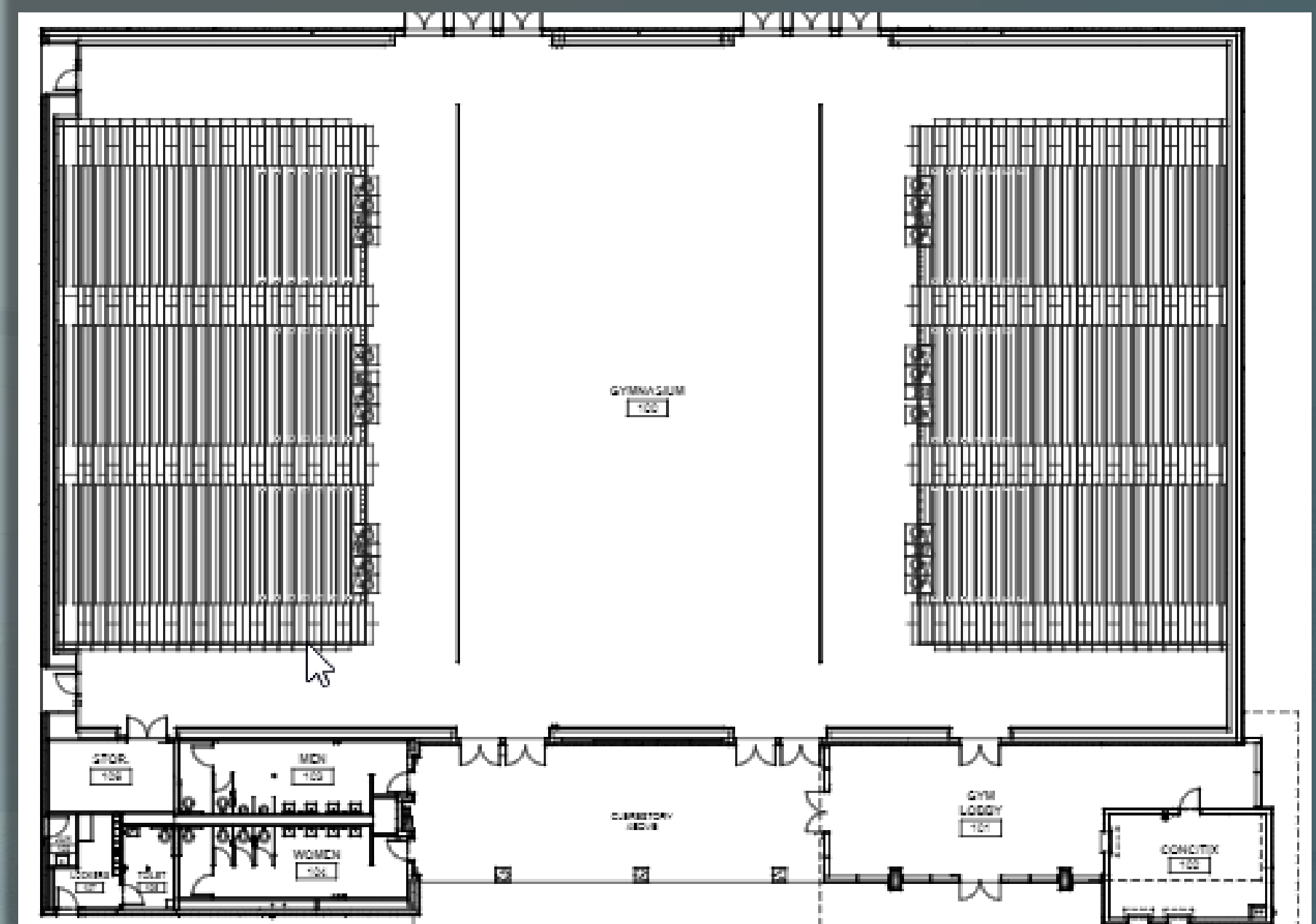
FLOOR PLAN WITH BLEACHERS OPEN
