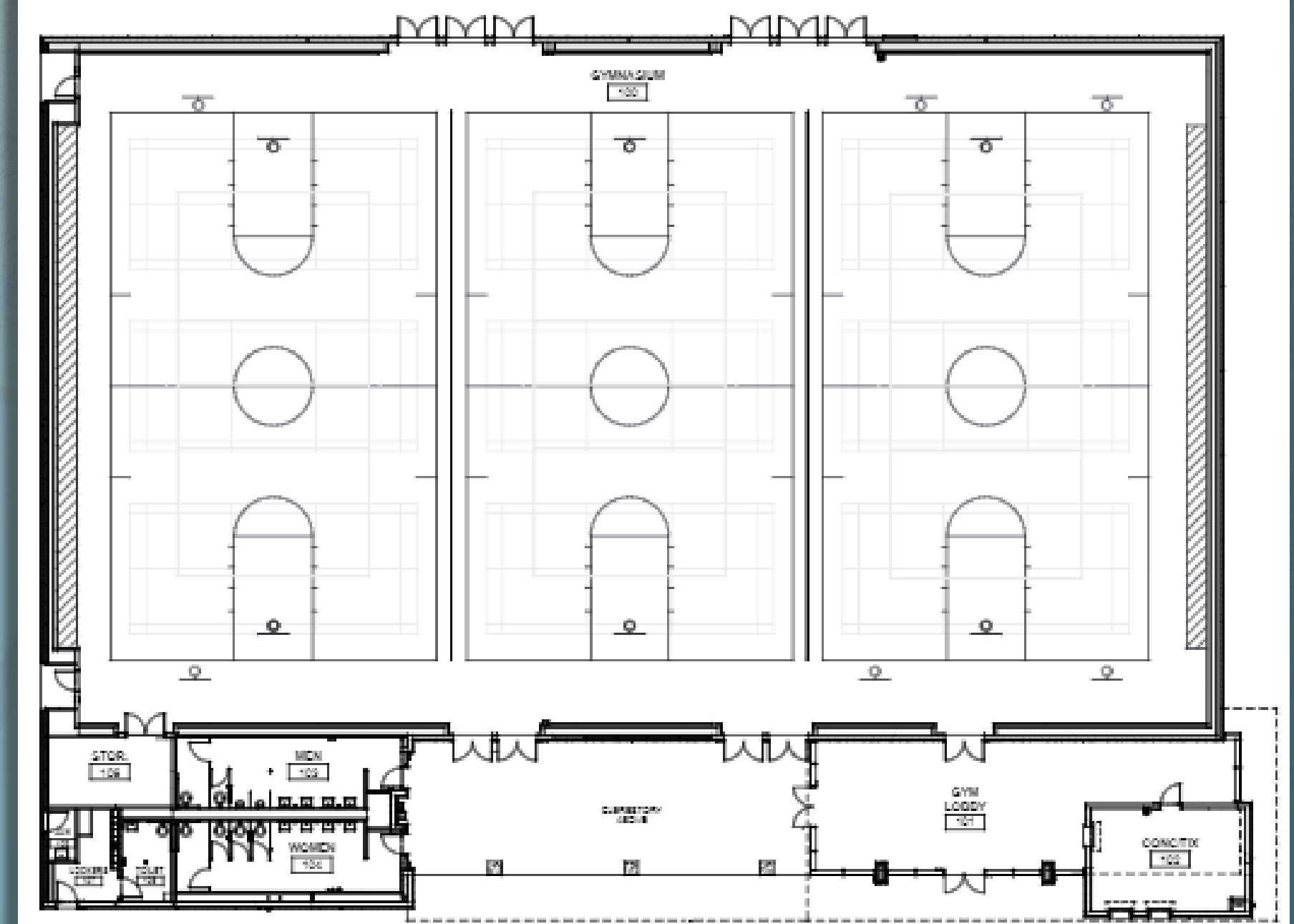
FLOOR PLAN WITH BLEACHERS OPEN
