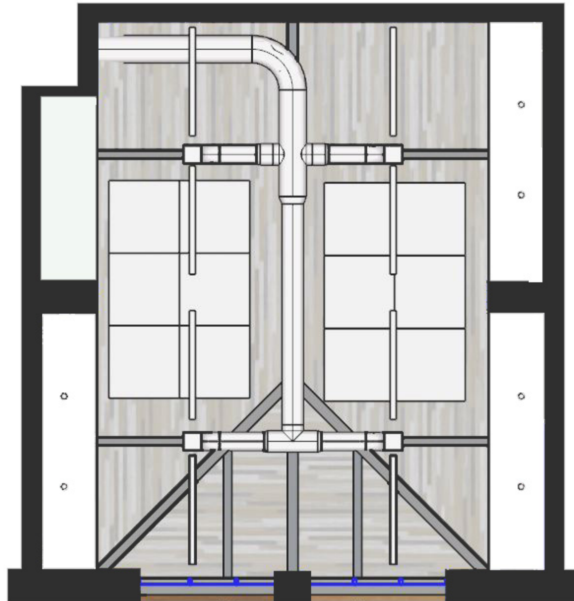
Acoustic Panel Composition Armstrong, Invisacoustics 'White' Individual Panel Size 2' x 4' Overall Panel Size 8' x 12' Direct Attach NRC 0.75
