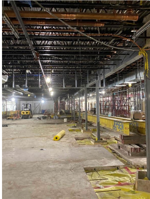
SFMS – Lower C&D shoring and structural steel
