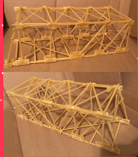
Model Pratt Truss Bridge Spaghetti & Linguini
